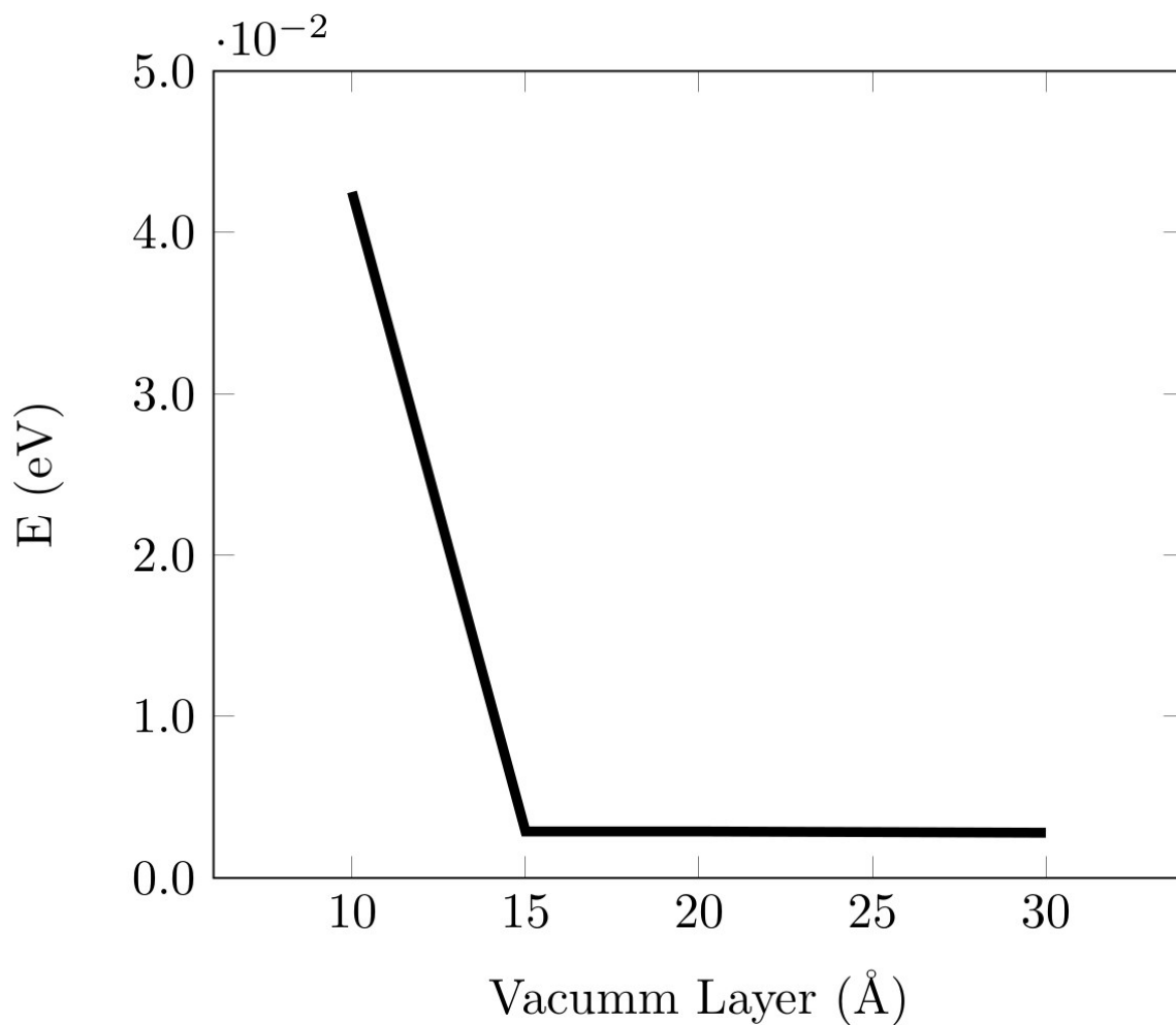
Figure S1: Vacuum layer convergence test regarding the adsorption energy variation of intermediate species (*OOH) over the ceria surface.
