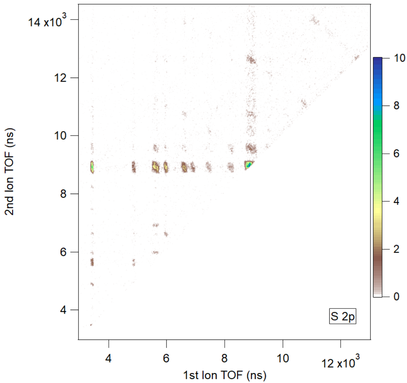
Fig. S 2 PIPICO map from S 2p PEPIPICO experiment
