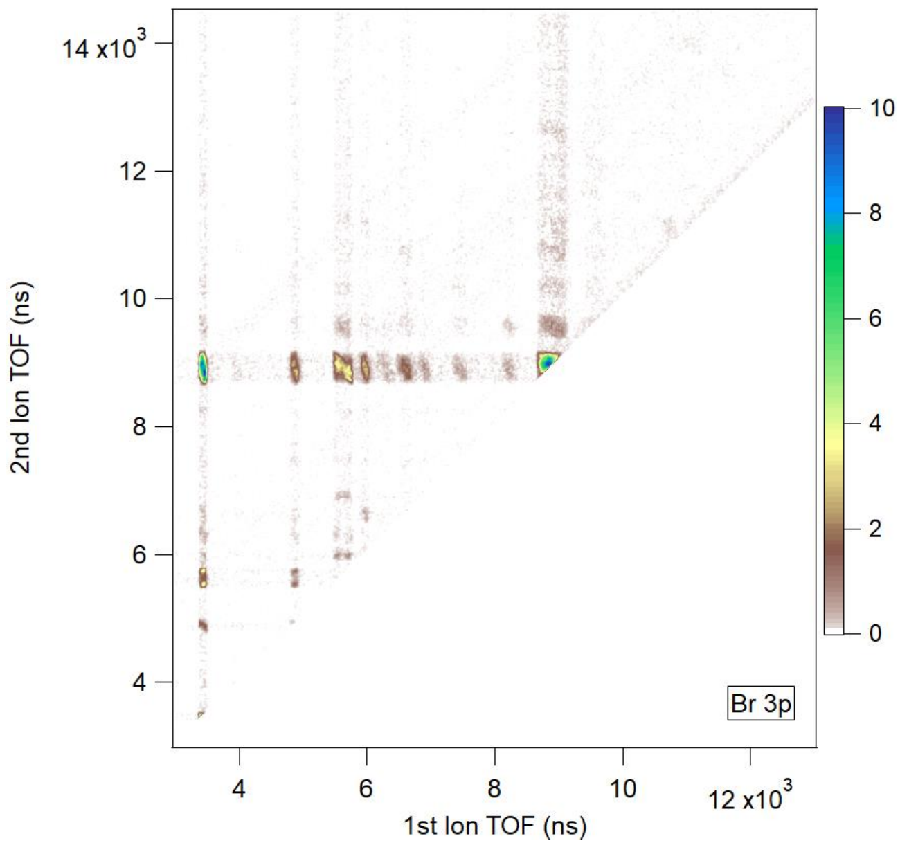
Fig. S 3 PIPICO map from Br 3p PEPICO experiment
