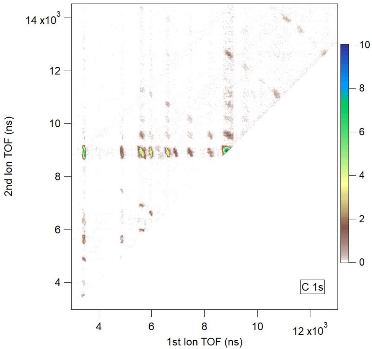
Fig. S 1 PIPICO map from C 1s PEPIPICO experiment
