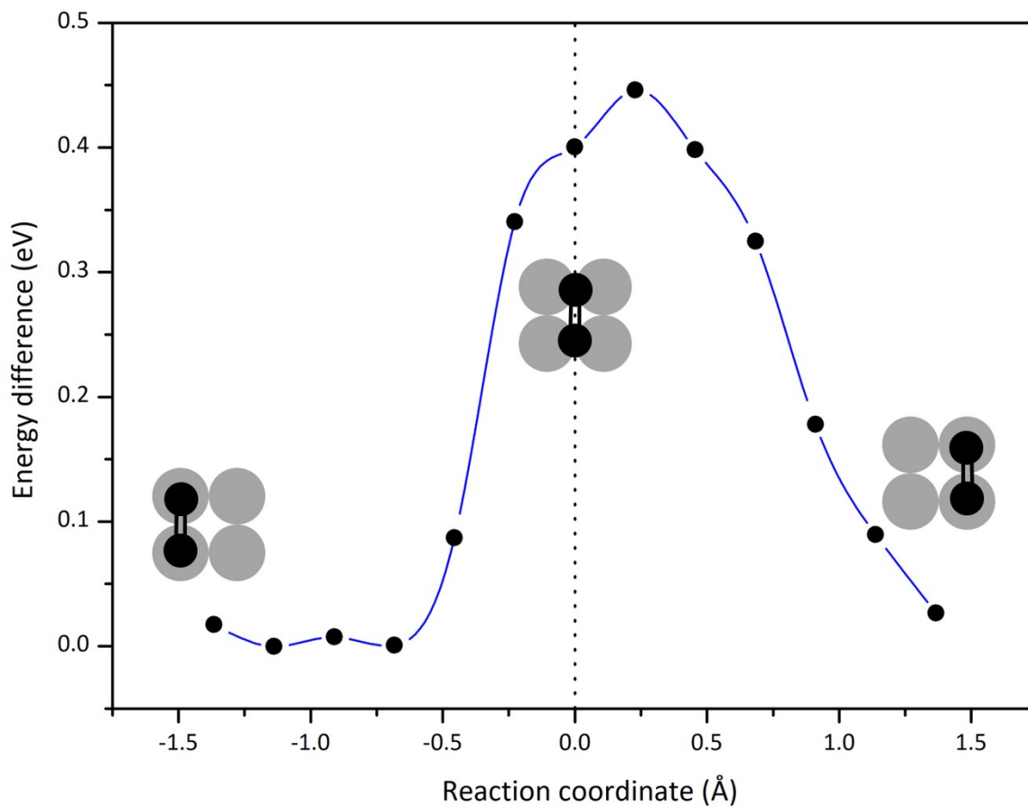
Figure S1: Energy barrier for the migration of the 1-pentene molecule on a (100) facet of a Pd 561 NP.
