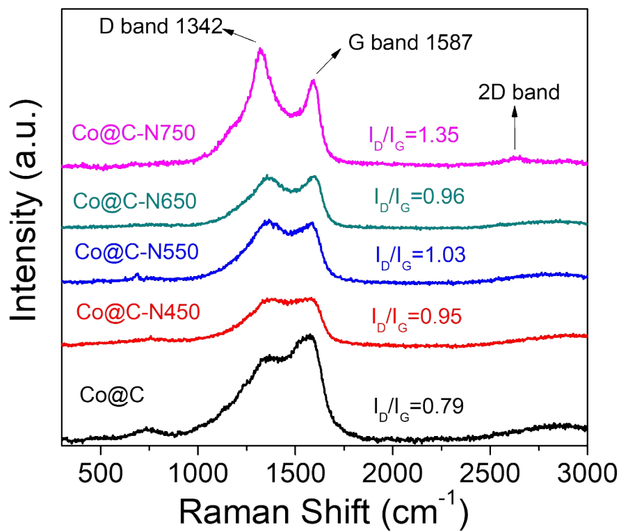
Figure S1 Raman spectrum of Co@C, Co@C-N450, Co@C-N550, Co@C-N650 and Co@C-N750
