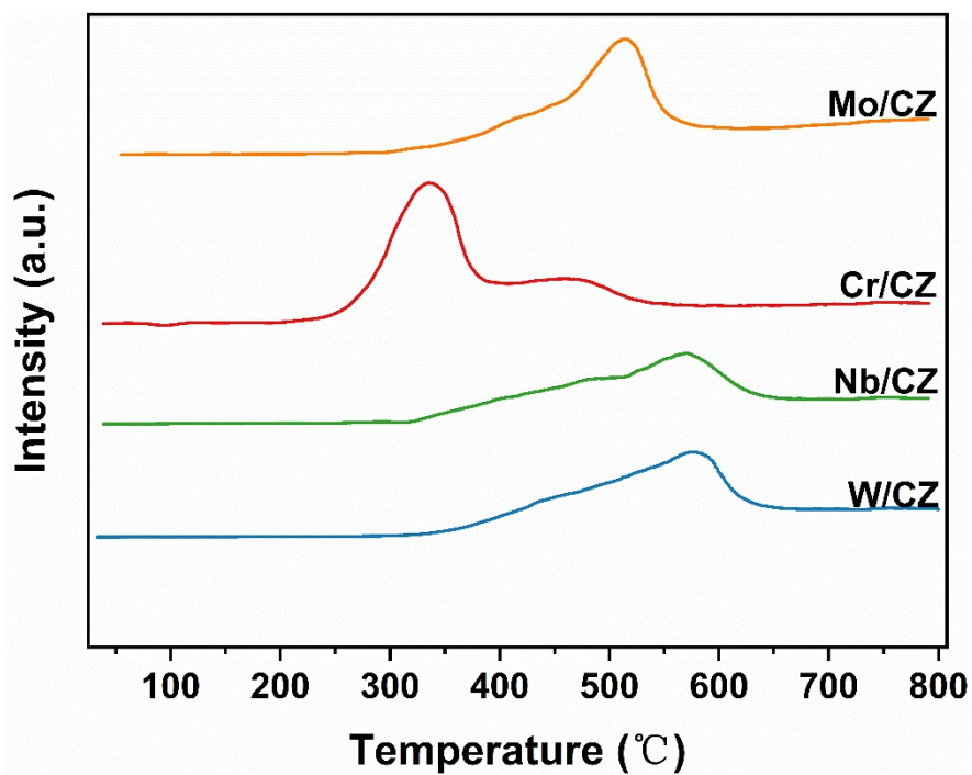
Fig. S1 The H 2 -TPR profiles of Mo/CZ, Cr/CZ, Nb/CZ, and W/CZ catalysts.
