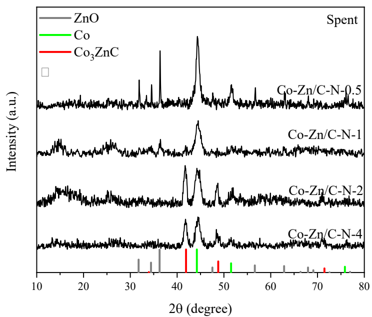
Fig. S4 XRD patterns of Co-Zn/C-N catalyst after reaction
