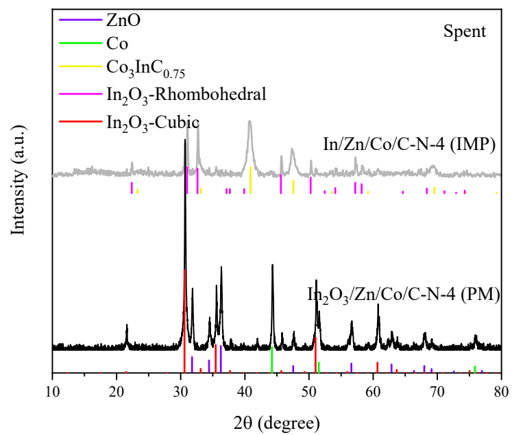
Fig. S6 XRD patterns of spent In-Co-Zn/C-N catalyst
