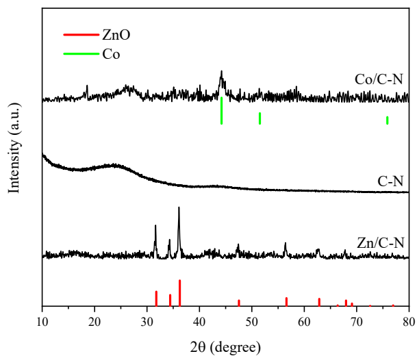
Fig. S3 XRD patterns of Co/C-N, Zn/C-N and C-N
