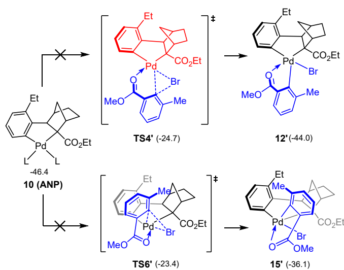
Fig. S2 Calculated Gibbs energy profiles for other two oxidative addition of aryl bromide on Pd(II).
