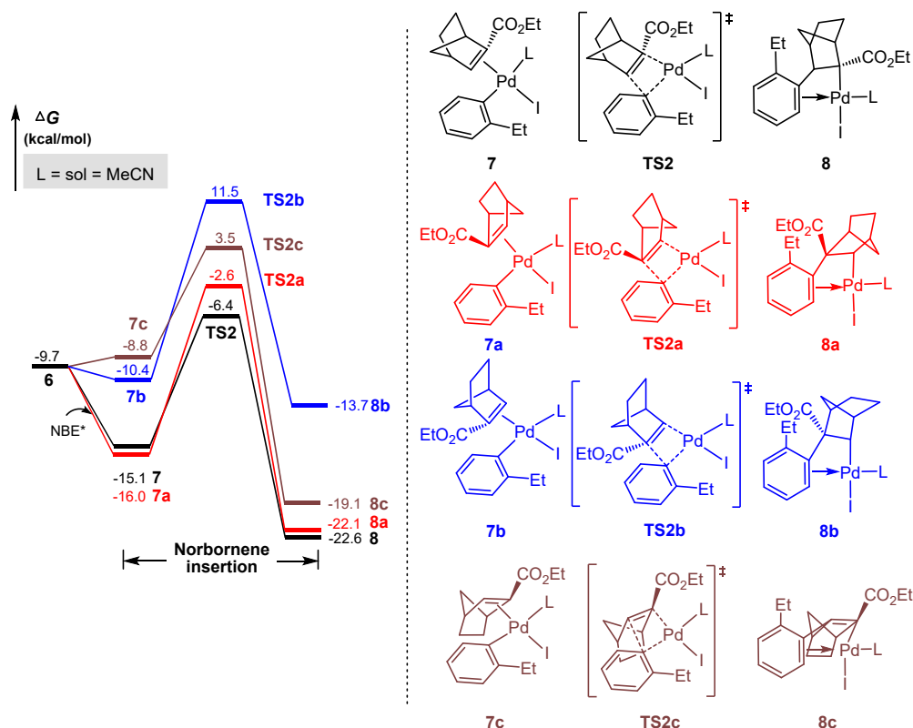
Fig. S1 Calculated Gibbs energy profiles for potential pathways of NBE* insertion into Pd–C bond.
