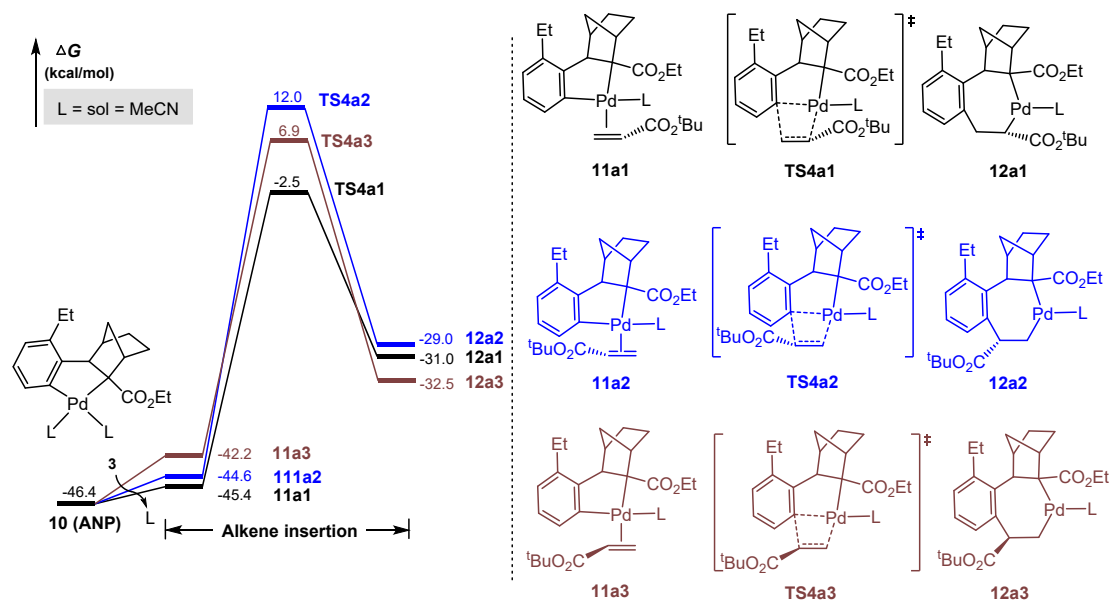
Fig. S3 Calculated Gibbs energy profiles for tert -butyl acrylate insertion into the Pd–C phenyl bond.
