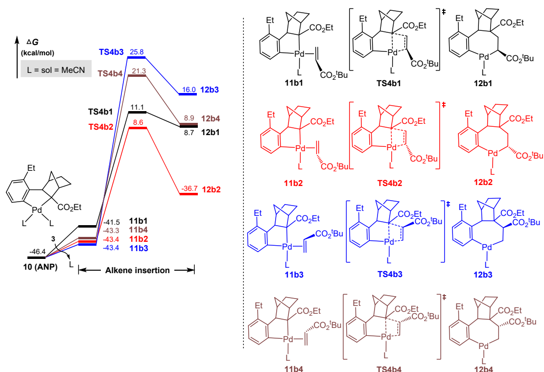
Fig. S4 Calculated Gibbs energy profiles for tert -butyl acrylate insertion into the Pd–C norborneyl bond.
