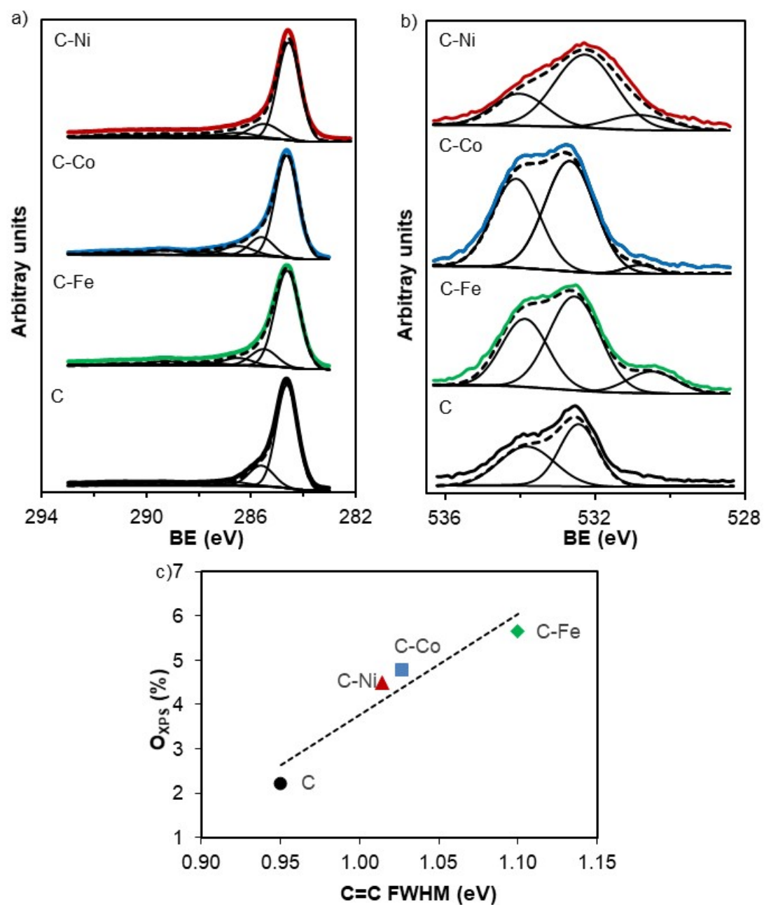
Figure S2. XP Spectra of a) C1s and b) O1s regions and c) correlation between FWHM (C=C) and the surface oxygen content.
