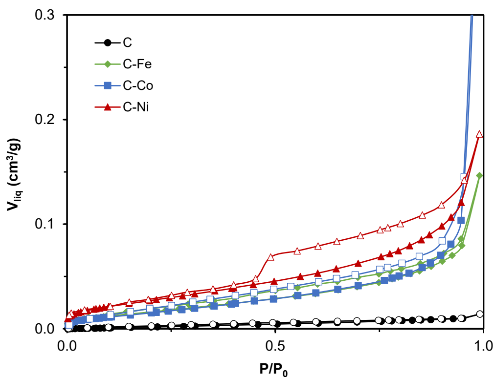
Figure S1. N 2 adsorption-desorption isotherms of samples.
