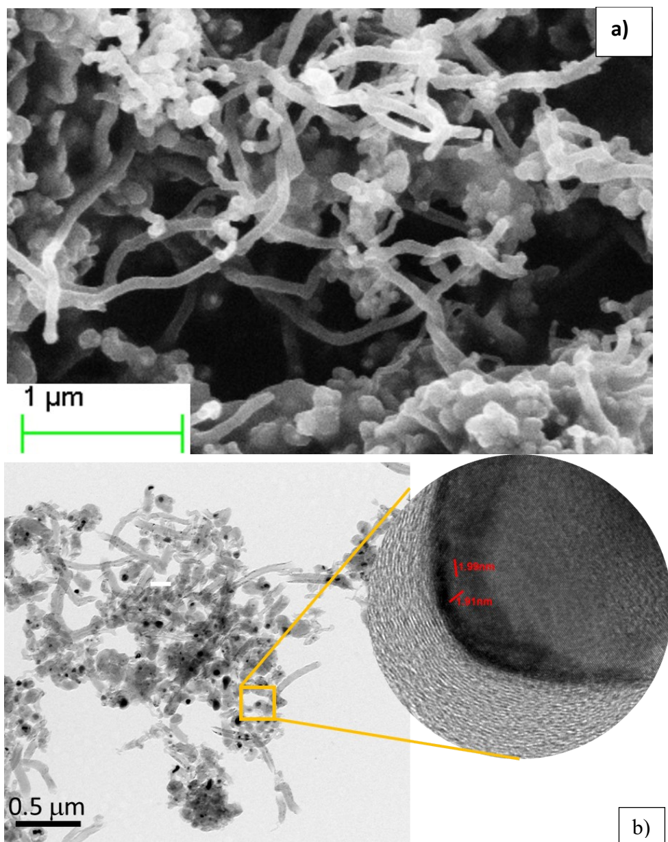
Figure S3. a) SEM and b) HRTEM images of C-Co samples after the catalytic test.
