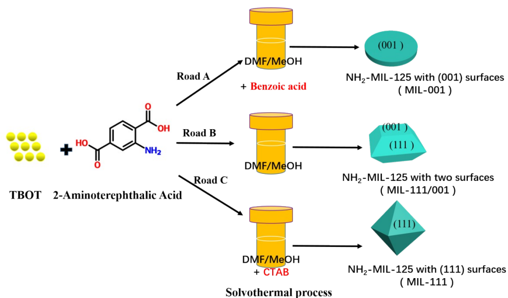
Fig. S1. Prepared process of Ti-MOFs
