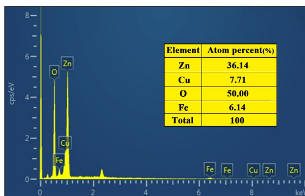
Fig. S1 The corresponding EDS spectrum of ZnO@CuO/ZnFe-LDH composite
