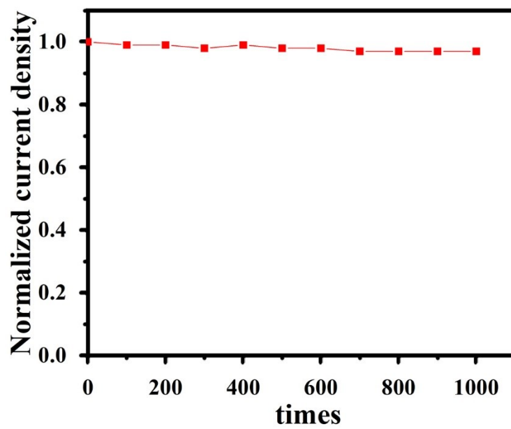
Fig. S3 Cycling stability measurement of ZnO@CuO/LDH photoanodes during 1000 cycles
