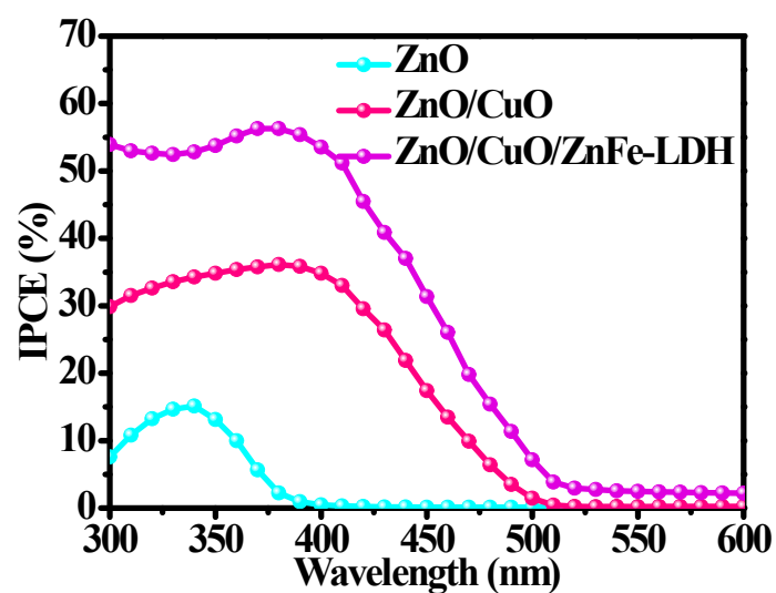
Fig. S2 Incident photon conversion efficiencies (IPCE) plots of ZnO NRs, ZnO@CuO NRs and ZnO@CuO/ZnFe-LDH composite
