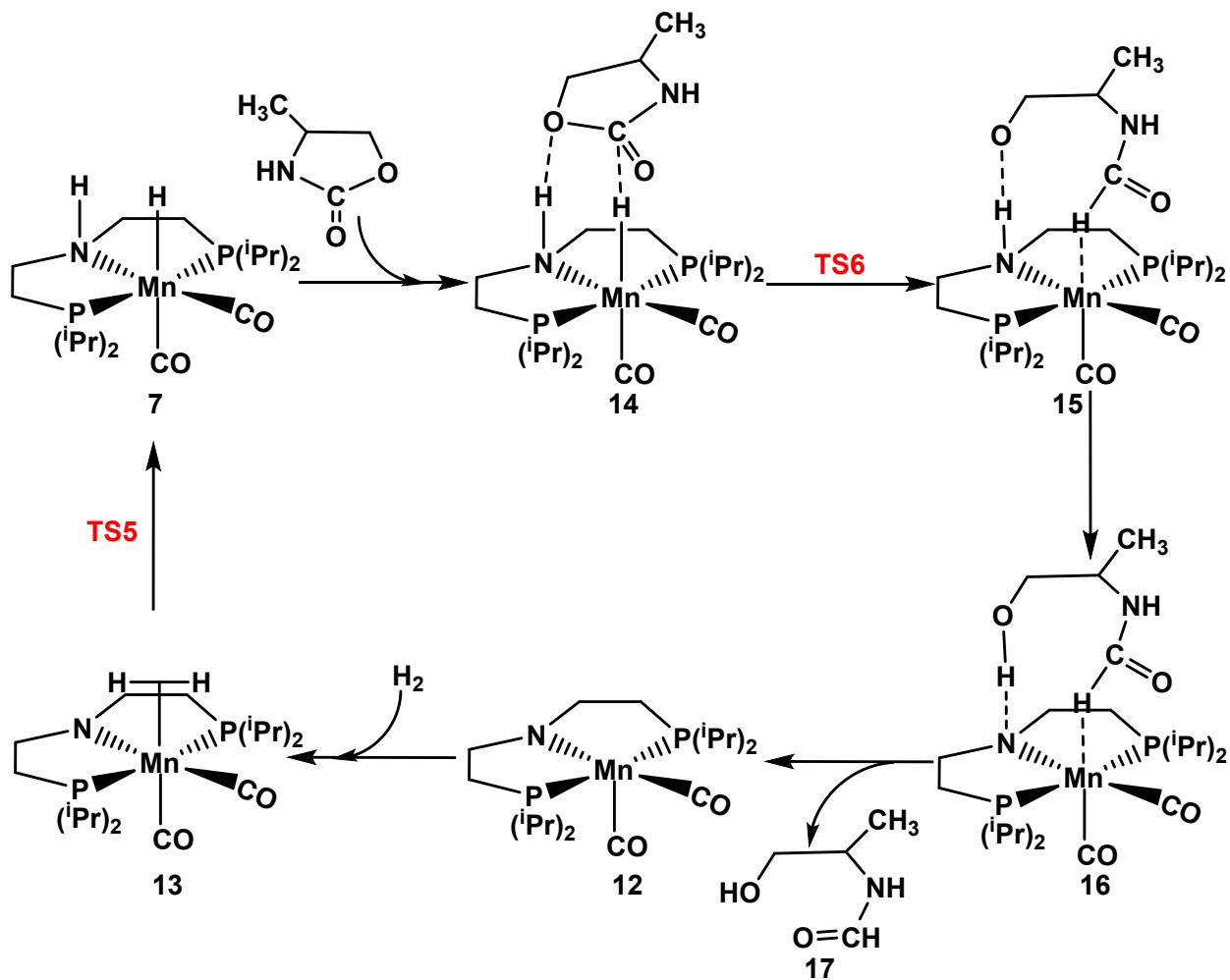
Scheme S2: Proposed mechanistic pathway of Pathway II for C–O bond cleavage of oxazolidinone by Mn(I)-PNP catalyst.
