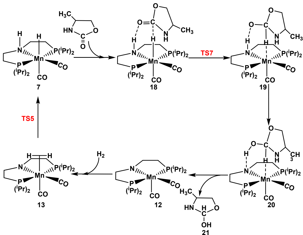
Scheme S3: Proposed mechanistic pathway of Pathway III for C=O bond hydrogenation of oxazolidinone by Mn(I)-PNP catalyst.
