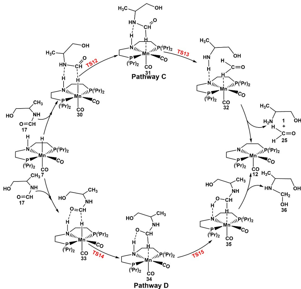
Scheme S4: The reaction mechanisms of C-N bond cleavage (Pathway C) and C=O bond hydrogenation (Pathway D) of (1-hydroxypropan-2-yl)formamide ( 17 ) to formaldehyde ( 25 ) and 2-((hydroxymethyl)amino)propan-1-ol ( 36 ) in the presence of Mn(I)-PNP catalyst.
