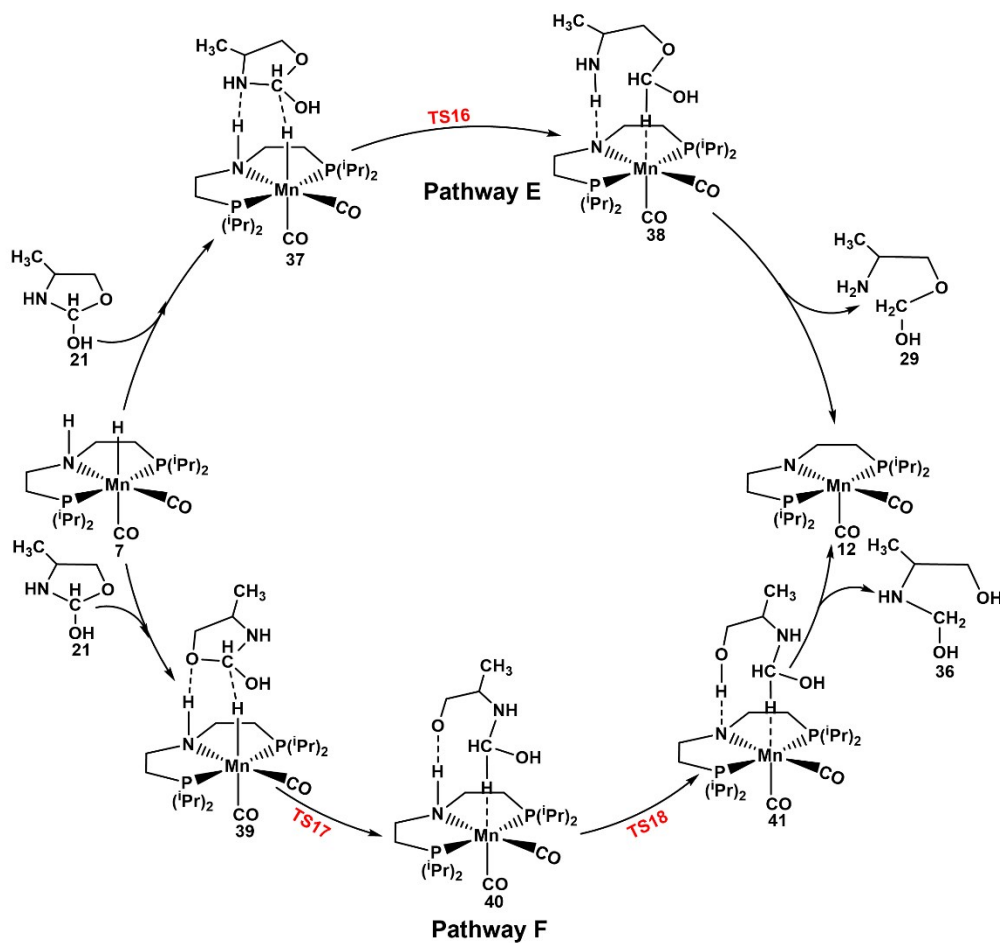
Scheme S5: Reaction scheme for C–N bond cleavage (Pathway E) and C–O bond hydrogenation (Pathway F) of 4-methyloxazolidin-2-ol ( 21 ) to (2-aminopropoxy)methanol ( 29 ) and 2-((hydroxymethyl)amino)propan-1-ol ( 36 ) in the presence of Mn(I)-PNP catalyst.
