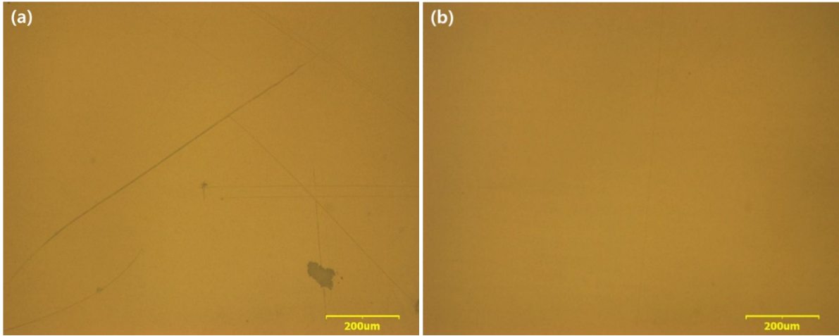
Figure S2. Optical microscopy images of (a) single \text{Al}_2\text{O}_3 and (b) structure B after bending test (5000 bending cycles with 3mm radius).
