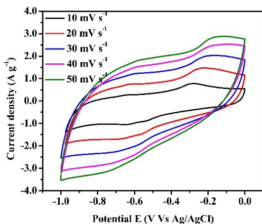
Fig. SI 1. The CV curves of N-rGO
