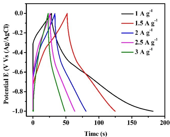
Fig. SI 2. The GCD curves of N-rGO
