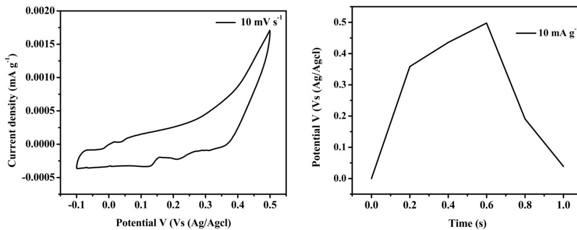
Fig. SI 4. The CV and GCD curves of the bare graphite sheet
