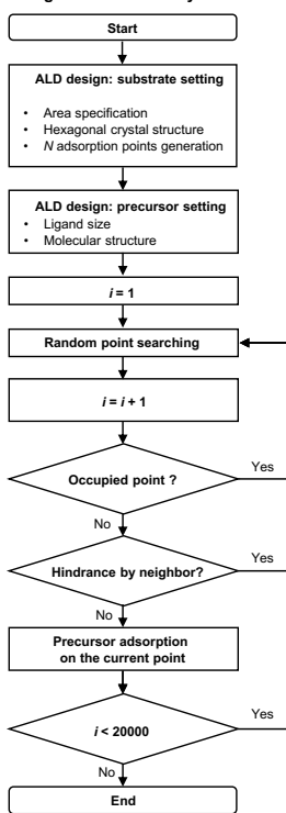
Algorithm : 1 st ALD cycle
