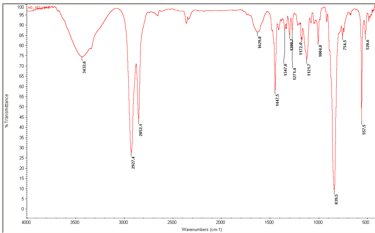
Figure S1: Infra-red spectrum of complex 1
