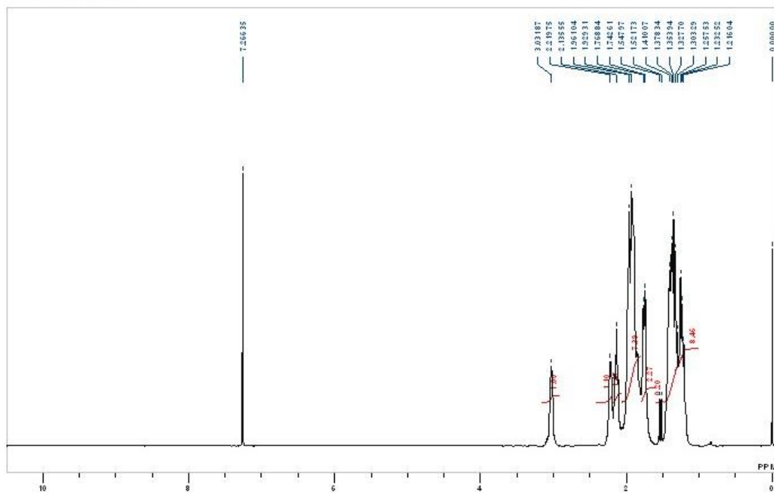
Figure S2: ^1\text{H} NMR spectrum of complex 1 in \text{CDCl}_3 .
