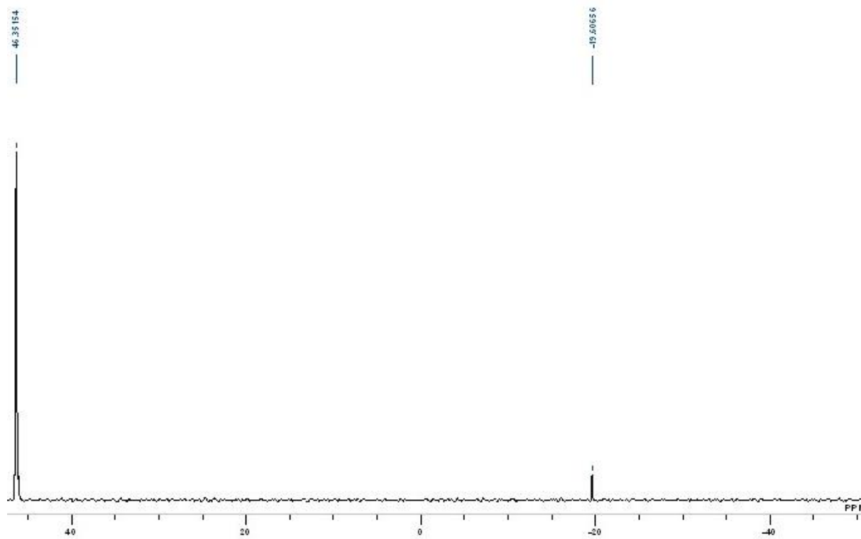
Figure S4: ^{31}\text{P} NMR spectrum of complex 1 in \text{CDCl}_3 .
