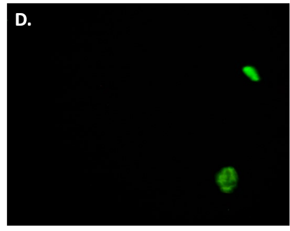
ZnS:Cd
