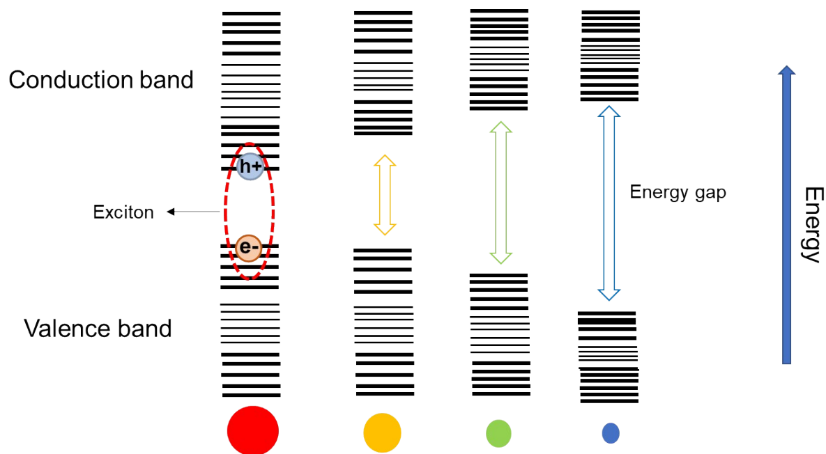
Figure S 1: schematic representation of QDs' size variation and exciton radius.
