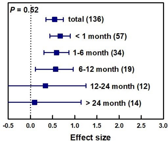
(c) Post-fire duration
