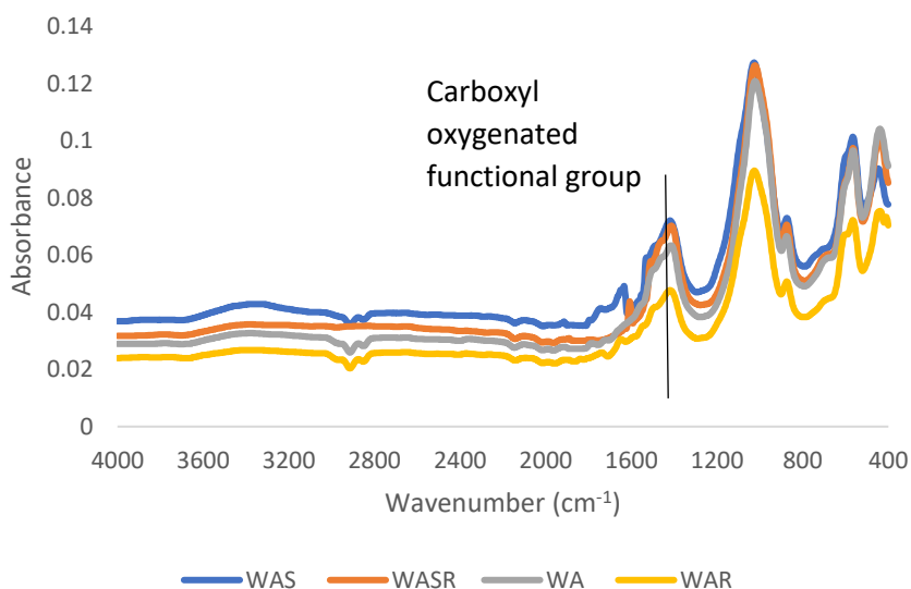
SI 4 – FTIR spectra of larch biochar sintered with wood ash before rinsing with deionised water (WAS) and after rinsing with 800mL of deionised water (WASR) and larch biochar mixed cold with wood ash before rinsing with deionised water (WA) and after rinsing with deionised water (WAR)
