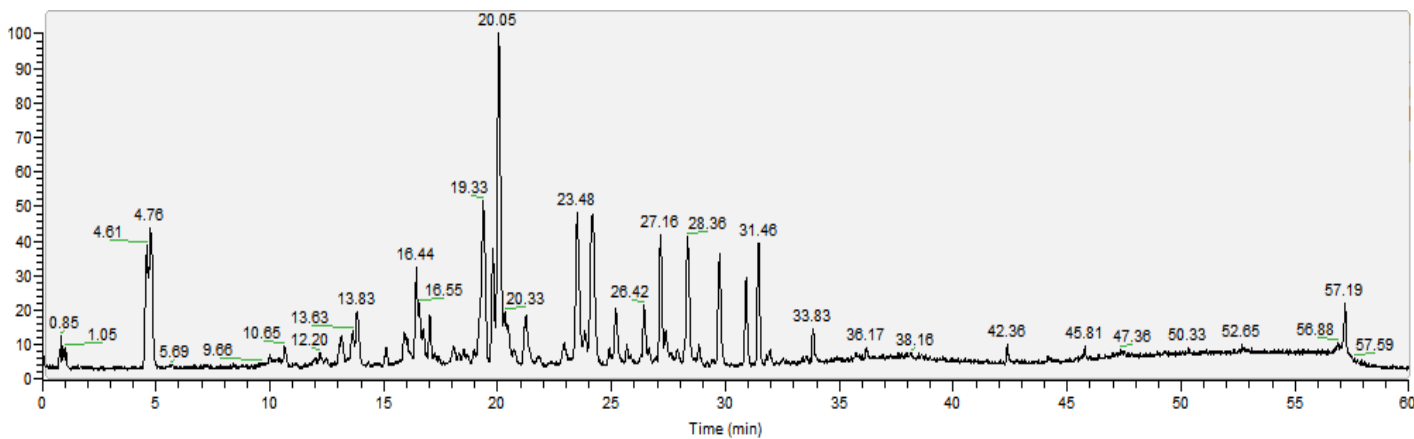
Electronic Supplementary Material (ESI) for Food & Function. Supplementary Figure 1 The total ion current (TIC) chromatogram of the compounds identified in TB-TF.
