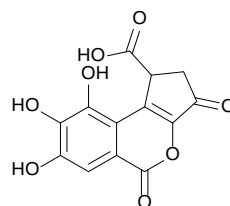
brevifolin carboxylic acid
