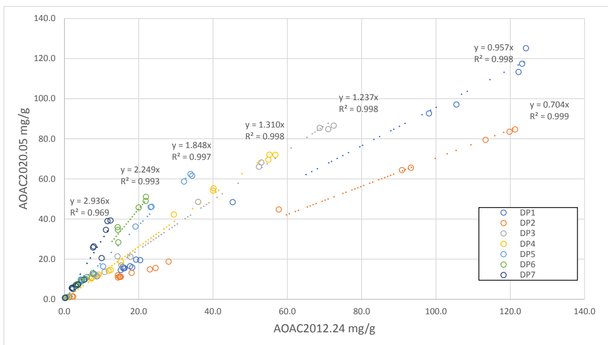
Figure S2. Comparison of individual DP contents measure with AOAC2012.24 and AOAC2020.05 in mg/g. Linear regression, forced through origin show the bias associated with each DP for DP1-7.
