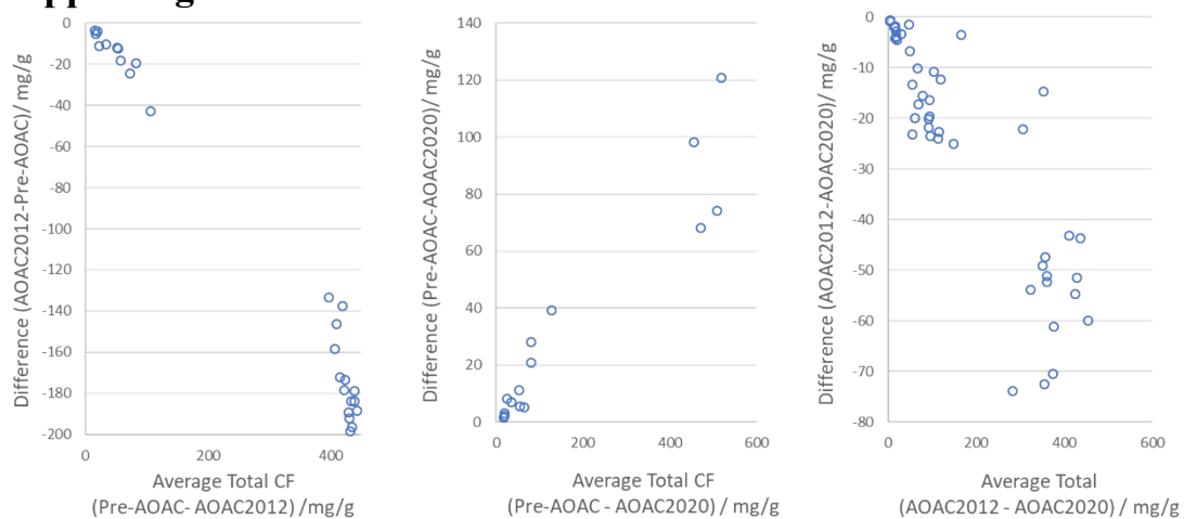
Figure S1. Relative differences between total CF determined by two methods against as a function of the total CF determined by two methods.
