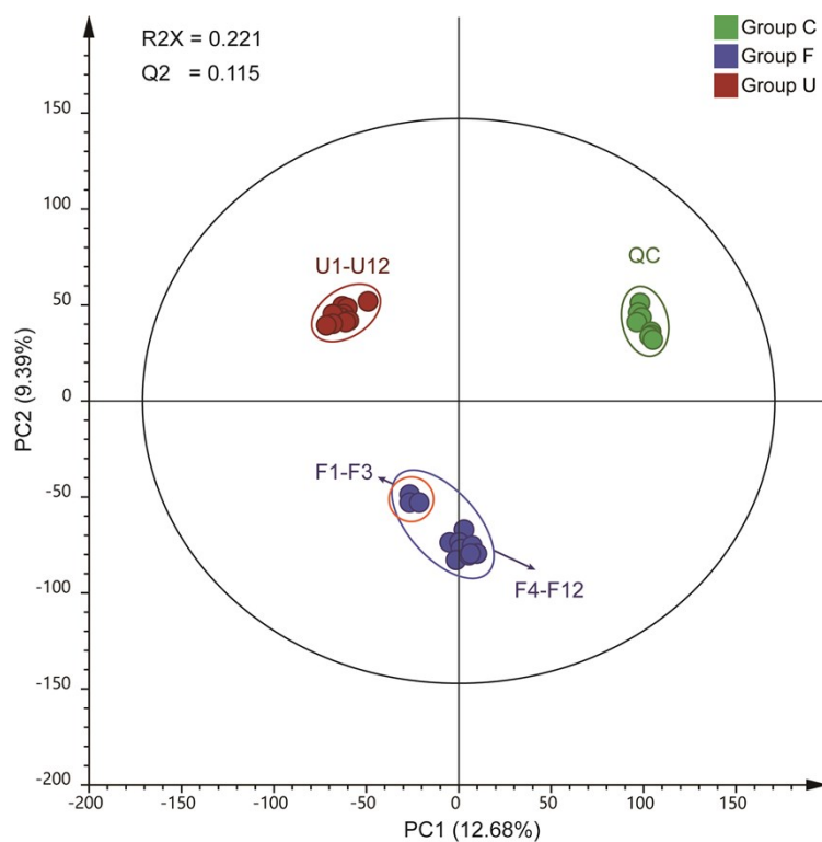
S Figure 2. PCA scores scatter plot of unfermented material samples (group U), fermented samples (group F) and quality control samples (group C). Three samples with 1-year fermentation time were extra encircled by orange circle in group F.
