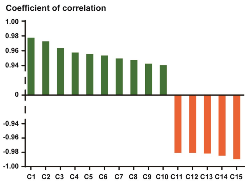
S Figure 4. Coefficient of correlation between 15 discriminant metabolites and \alpha -glucosidase inhibition.
