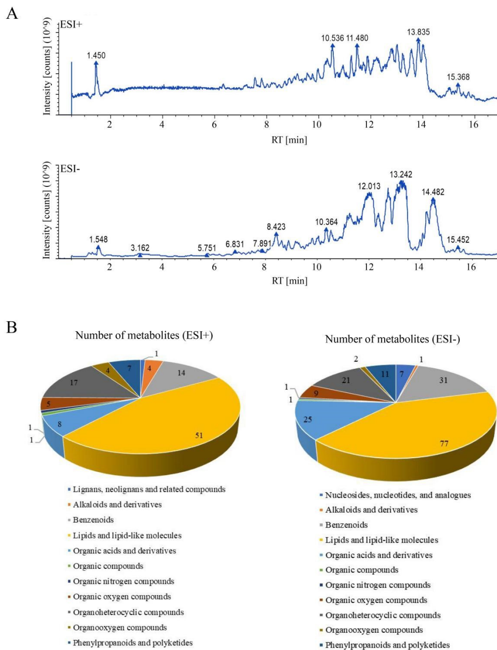
Fig. S2 The BRPS identified by LC-MS. (A) TIC diagram for different ion modes of BRPS. (B) Composition identification in different ionic modes of BRPS.
