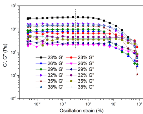
Fig.S2 Strain sweep of hierarchical emulsion at 25 °C (a fixed frequency of 1 Hz).
