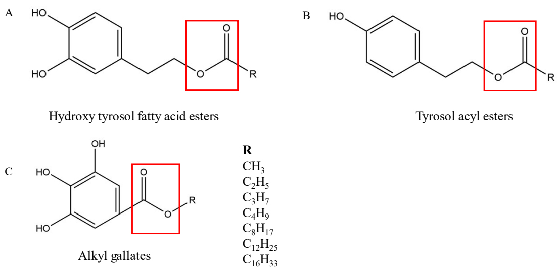
Fig.1S Structures of hydroxytyrosol acyl esters (A), tyrosol acyl esters (B) and alkyl gallates (C).
