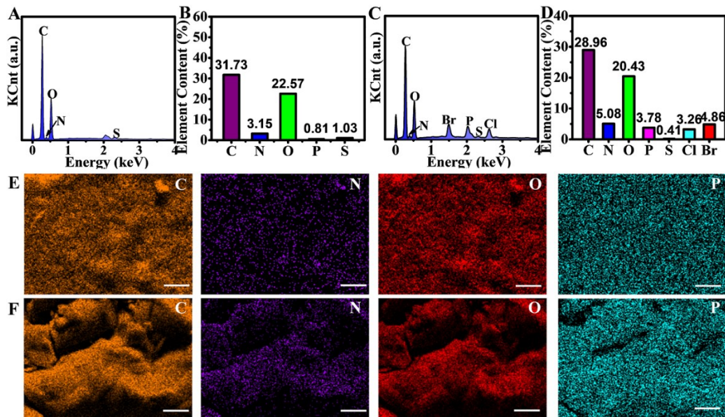
Fig. S1. EDS spectra, element content and elemental mapping images of WPI-DX (A,B,E) and TPP-WPI-DX (C,D,F).
