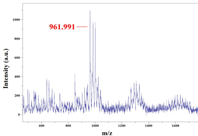
Figure. S1 MALDI-TOF-MS spectrum of UPFNs from Undaria pinnatifida .
