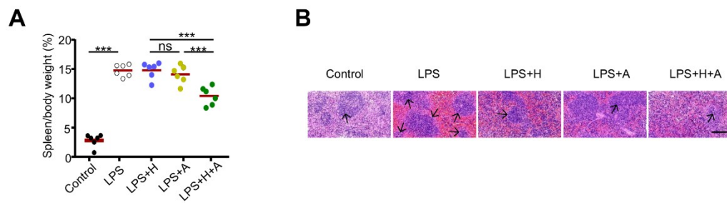
Supplementary Figure 3 Graph shows the ratio of spleen/ body weight of mice in each group (A). The infiltration of immune cells in spleen (B) was examined by H&E staining, scale bar=250 \mu m.
