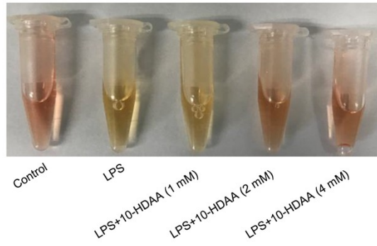
Supplementary Figure 2 The color of cell culture medium after different treatments.
