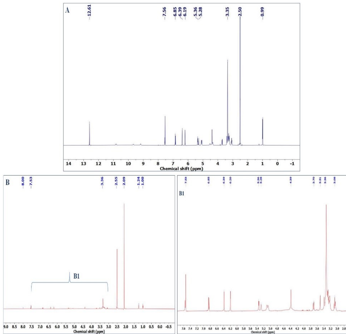
Fig. S2 ^1\text{H-NMR} spectra of (A) pure rutin and (B) rutin nanorods. (B1 correspond to ^1\text{H-NMR} signals of rutin nanorods).
