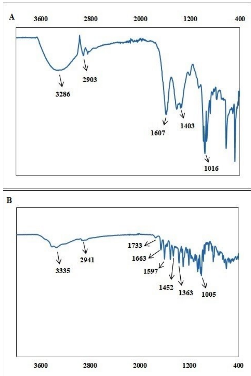
Fig. S1 FTIR spectra of (A) pure rutin and (B) rutin nanorods.
