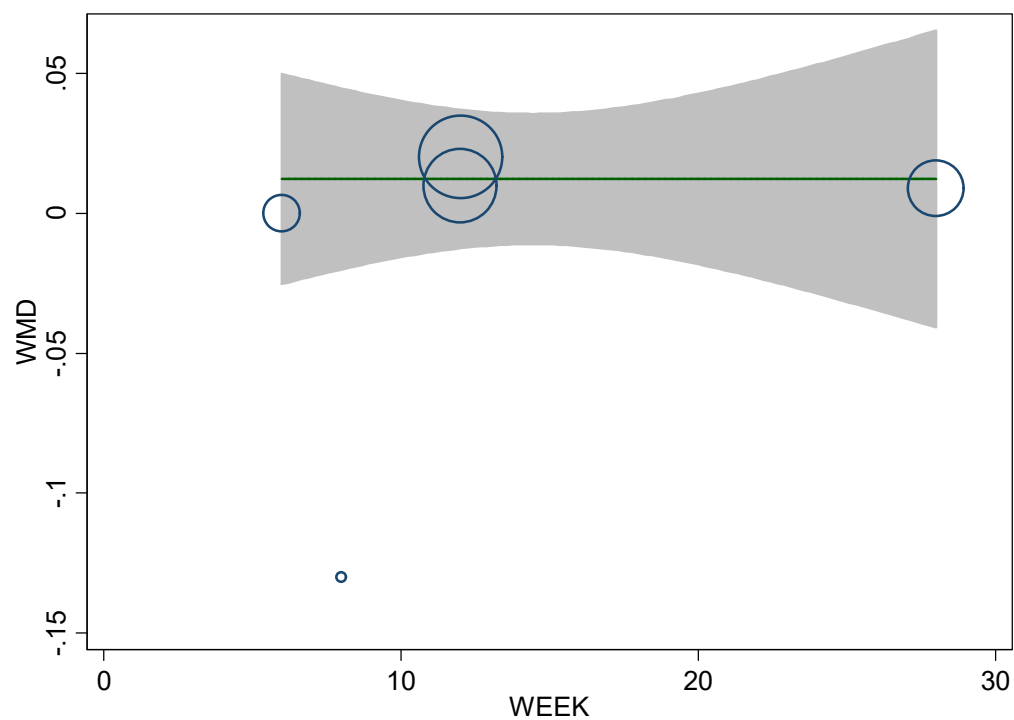
Supplemental Figure 31 The results regression analysis of QUICKI effect and intervention time.
