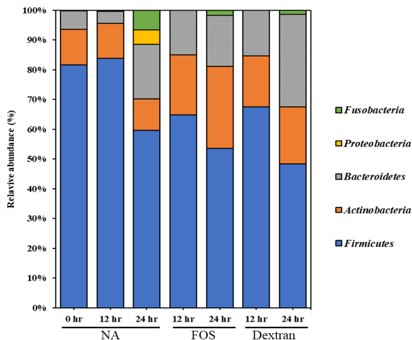
Supplementary Figure 1. Bacterial taxonomic compositions at phylum level after in vitro fecal fermentation. NA, no substrate addition; FOS, addition of fructooligosaccharide; Dextran, addition of Leuconostoc mesenteroides SPLC742 dextran.
