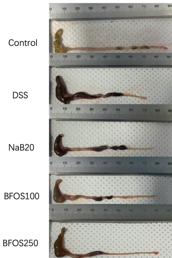
Figure S3. Macroscopic appearance of colon in the DSS-induced colitis of mice.
