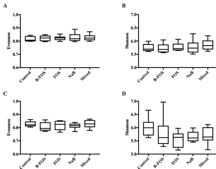
Figure S1. Comparison of alpha diversity indices amongst groups before and after 4-week oral administration. Alpha diversities of microbial communities are shown as evenness at 0 week (A) and the fourth week (C) and richness at 0 week (B) and the fourth week (D). Significance was accepted as P < 0.05 ( n = 8 ).
