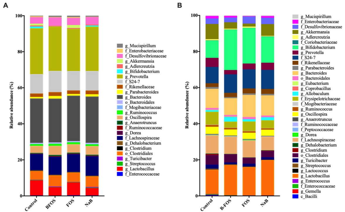
Figure S2. Microbiota composition of average relative abundance of each group at genus level before (A) and after 4-week treatments (B). Taxa with relative abundance below 0.1% were excluded prior to analyses. (n = 8).
