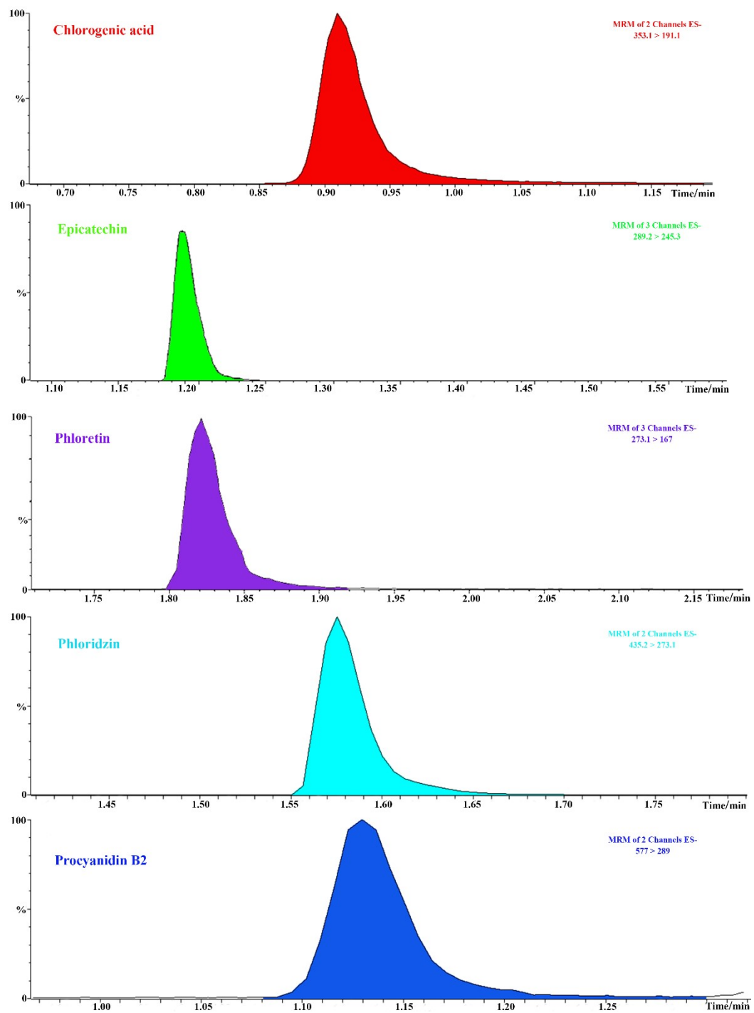
Supplementary Figure S1 LC-MS/MS chromatograms of the most abundant five phenolic compounds identified in apple phenolic extract (APE).
