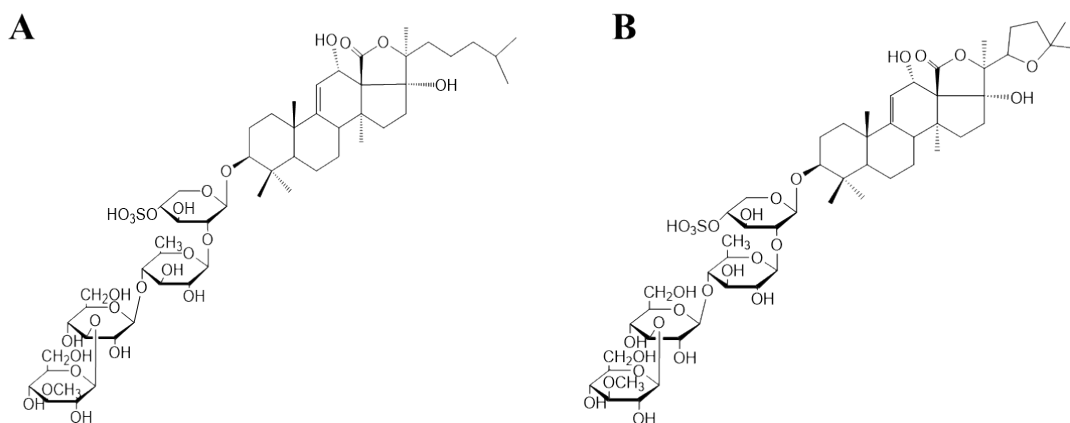
Supplementary Figure 1. The structure of Echinaside A (A) and Holothurin A (B)
