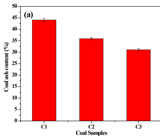
Fig. 1 Calculated ash contents of three coal samples in terms of combined concentrations of oxides of Na, Mg, Al and Si
