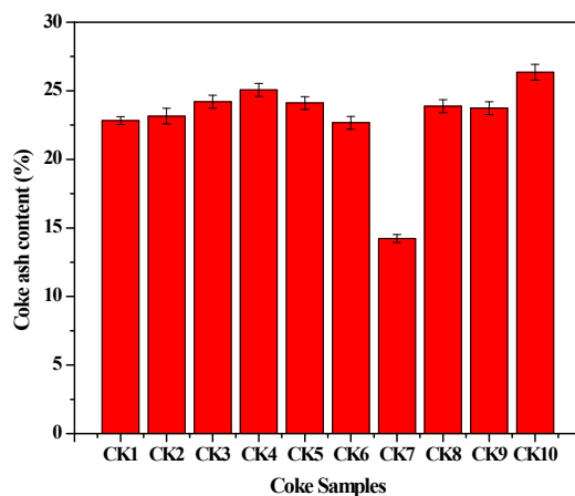
Fig. 2 Determination of ash contents in terms of combined concentrations of oxides of Na, Mg, Al and Si for ten coke samples (CK1 – CK10)
