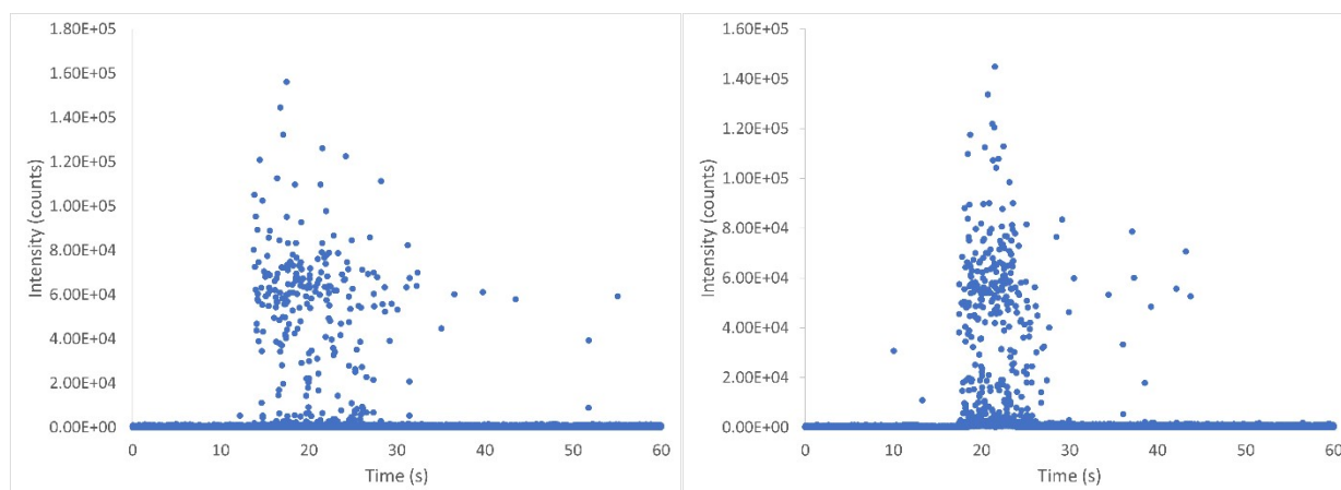
Fig. S1 Temporal profiles obtained for one injection of Au NPs suspension by FI-spICPMS (left) and MSFA-spICPMS (right) with a new injection valve
