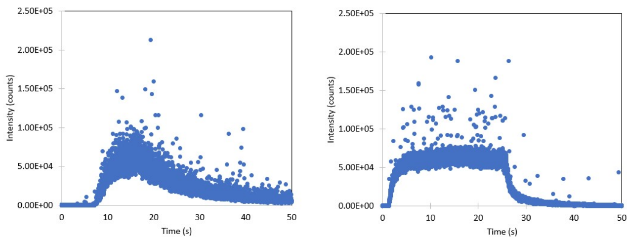
Fig. S2 Temporal profiles obtained for one injection of 5 \mu\text{g L}^{-1} Au solution by FI-spICPMS (left) and MSFA-spICPMS (right) with an old injection valve
