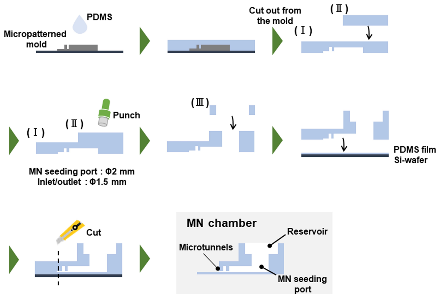
Supplementary Fig. 1 Fabrication process for the microdevice
