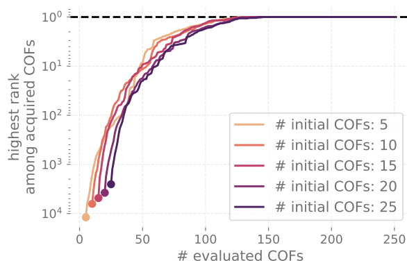
Figure S1: How does the number of COFs used to initialize the GP surrogate model for BO influence the search efficiency of BO? Here, we show the search efficiency curves of BO when initialized with different numbers of COFs (solid points).
