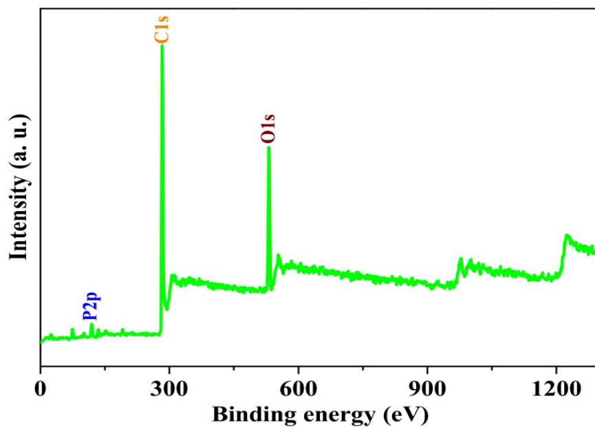
Figure S1 XPS survey spectrum of WSAC-3
