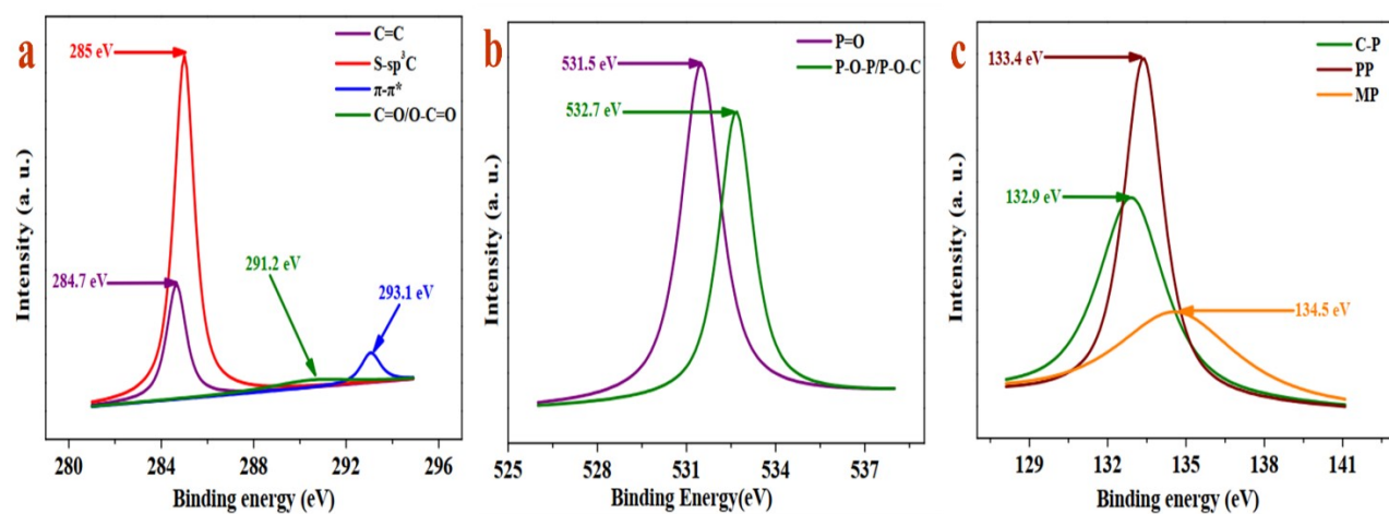
Figure S4 (a) High resolution C1s of WSC; (b) High resolution O1s of WSC; (c) High resolution P2p of WSC
