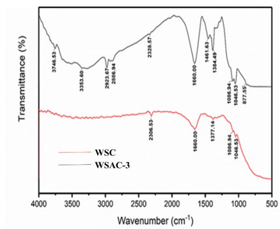
Figure S5 FT-IR spectra of WSC and WSAC-3 materials
