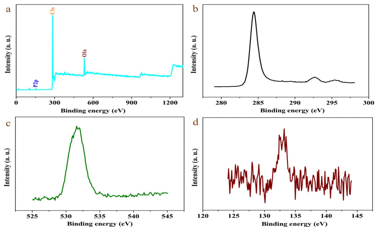
Figure S3 (a) XPS survey spectrum of WSC; (b) C1s scan of WSC; (c) O1s scan of WSC; (d) P2p scan of WSC
