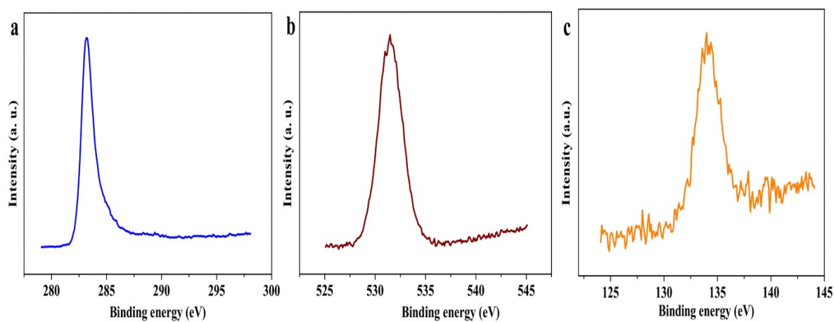
Figure S2 (a) C1s scan of WSAC-3; (b) O1s scan of WSAC-3; (c) P2p scan of WSAC-3
