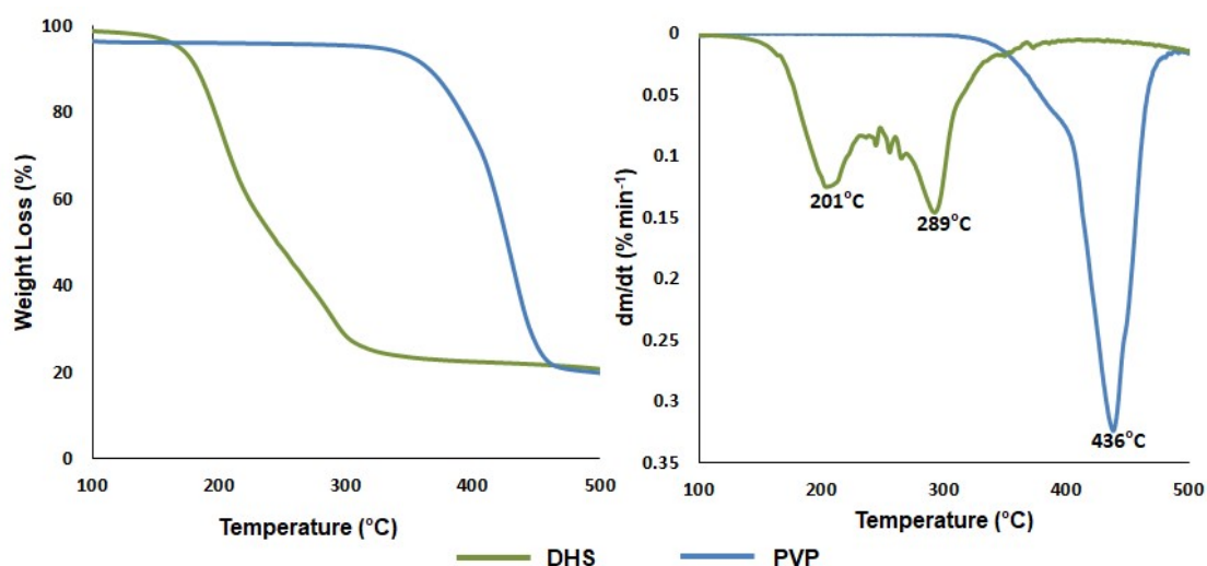
Figure S1: Graphs of thermogravimetric analysis (TGA) determining the decomposition temperatures of PVP and DHS.
