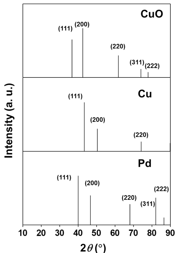
Figure S1. Simulated XRD lines for Pd, Cu and CuO.
