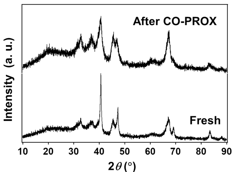
Figure S2. Comparison of pXRD profiles of the alloy PDCu catalyst before and after the CO-PROX reaction.
