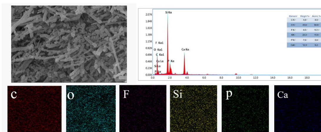
S2. FESEM-EDS mapping of the F-HAP-SiO 2
