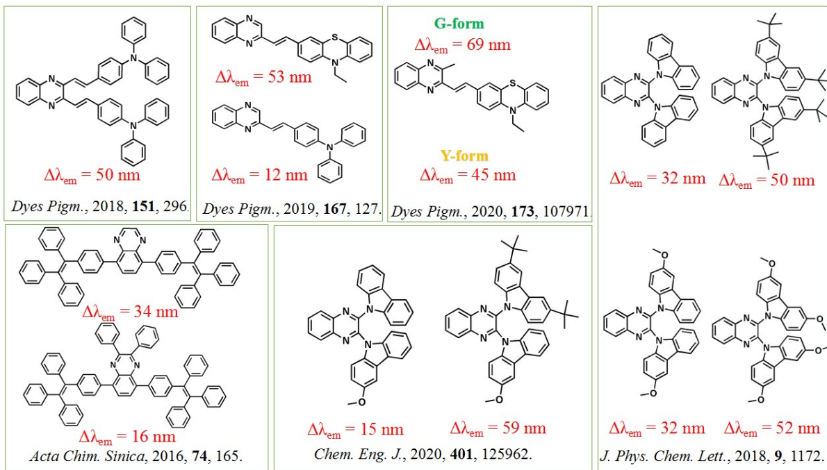
Fig. S1 MCL properties of quinoxaline-based fluorophores
