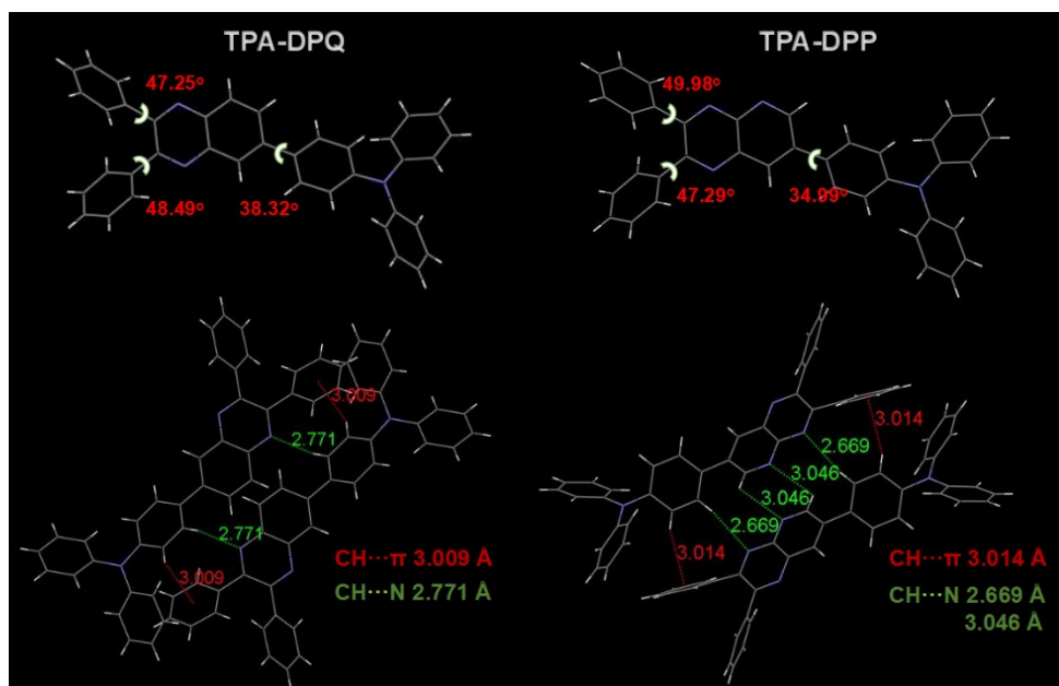
Fig. S2 The single crystal structures and molecular interactions of TPA-DPQ and TPA-DPP at 296 K
