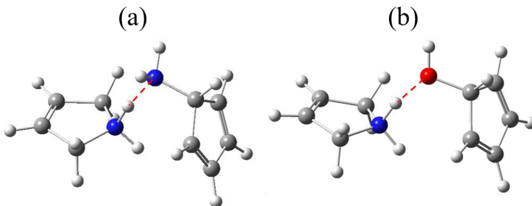
Figure S2. The optimized structures of the MCs for: (a) entry 2-1; and (b) entry 2-2. The red dashed lines indicate the HB interaction.
