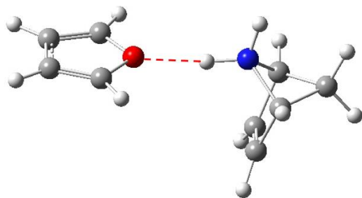
Figure S3. The optimized structure of the MC associated with the reactants of Scheme 3. The red dashed line indicates the HB interaction.
