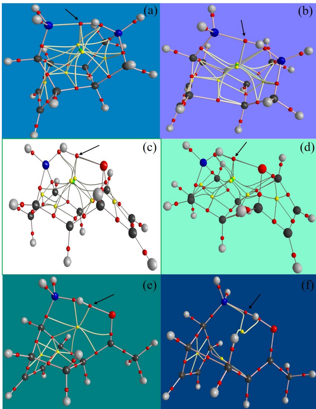
Figure S5. The results of the QTAIM analysis for: (a) exo cycloadduct corresponding to entry 2-1; (b) exo TS corresponding to entry 2-1; (c) exo1 cycloadduct corresponding to Scheme 3; (d) exo1 TS corresponding to Scheme 3; (e) exo cycloadduct corresponding to entry 3-1; and (f) exo TS corresponding to entry 3-1. Black arrows indicate the critical point corresponding to the HB interaction.
