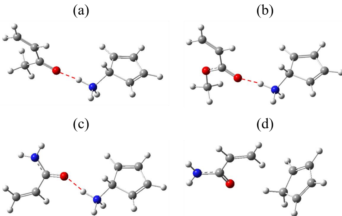
Figure S4. The optimized structures of the MCs for: (a) entry 3-1; (b) entry 3-2; (c) entry 3-3; and (d) entry 3-4. The red dashed lines indicate the HB interaction.
