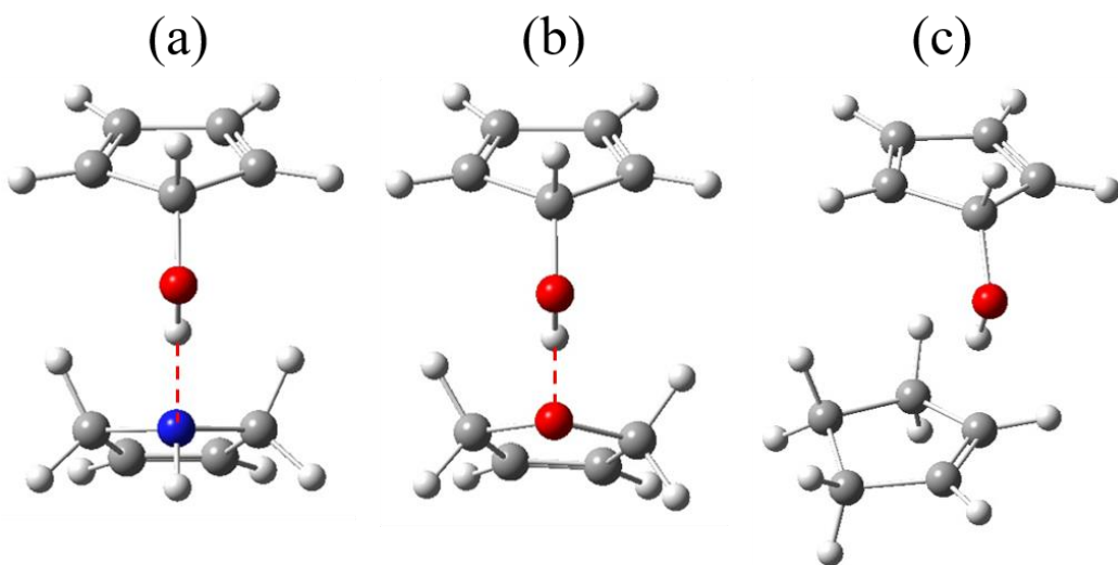
Figure S1. The optimized structures of the MCs for: (a) entry 1-1; (b) entry 1-2; and (c) entry 1-3. The red dashed lines indicate the HB interaction.
