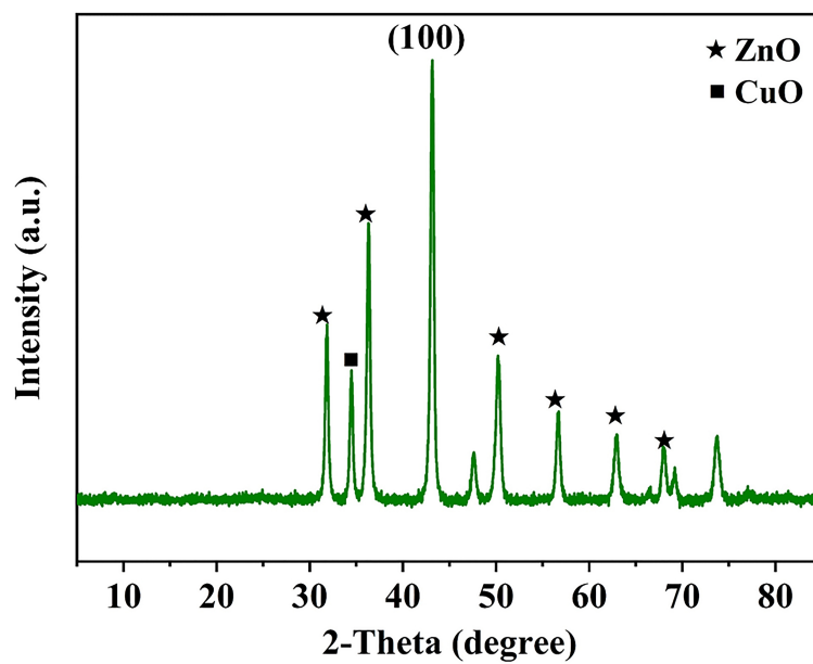
Fig. S1. XRD patterns of spent catalyst with the long time-on-stream of 10 h.
