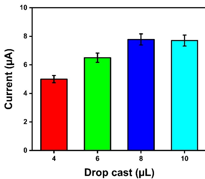
Fig. S2 CV response for loading amount (μL) of the \text{Fe}_2(\text{MoO}_4)_3/\text{SPCE} .
