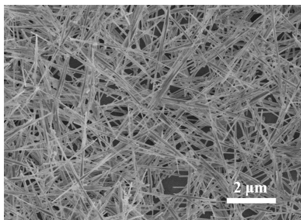
Fig. S1 SEM image of \text{Lu(OH)}_{1.63}\text{F}_{1.37} .
