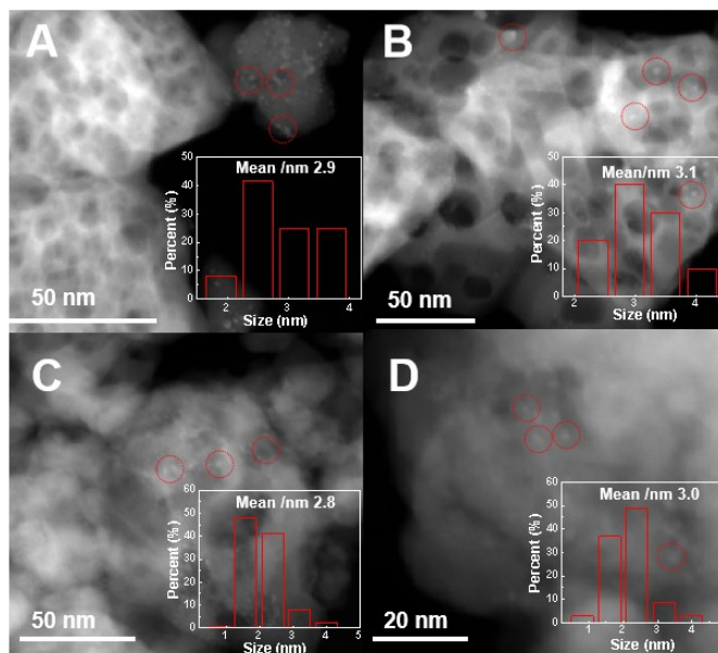
Fig. S1. HAADF-STEM of A) Pt/ZrO 2 , B) Pt-Mo/ZrO 2 , C) Mo/Pt/ZrO 2 and D) Pt/Mo/ZrO 2 catalysts (with particle size distribution of Pt inset).
