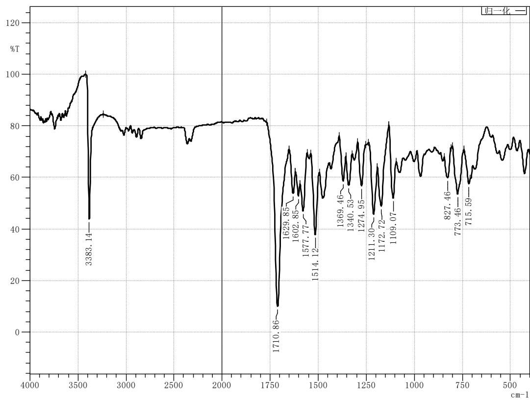
Figure 54 Infrared spectrum of compound M18
