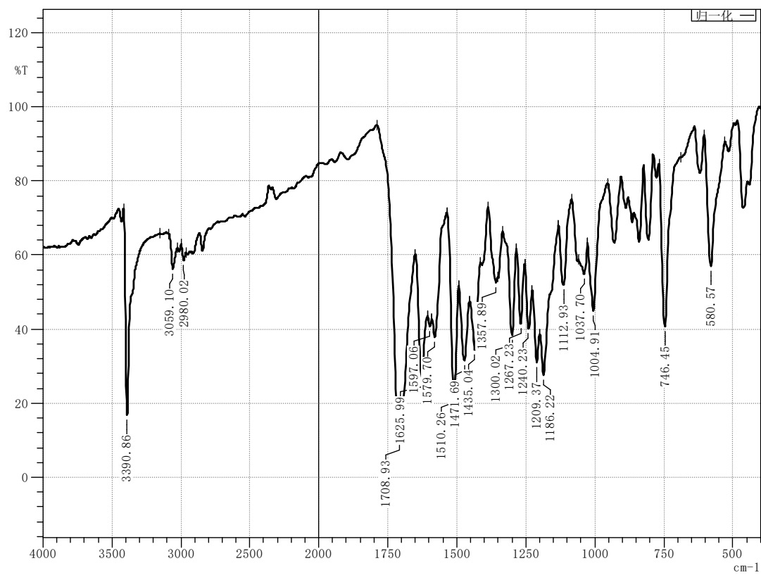
Figure 60 Infrared spectrum of compound M20
