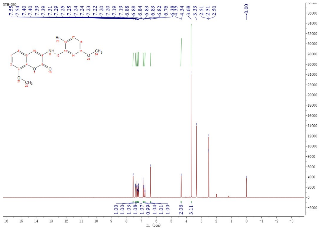
Figure 58 1 H NMR Spectrum of Compound M20
