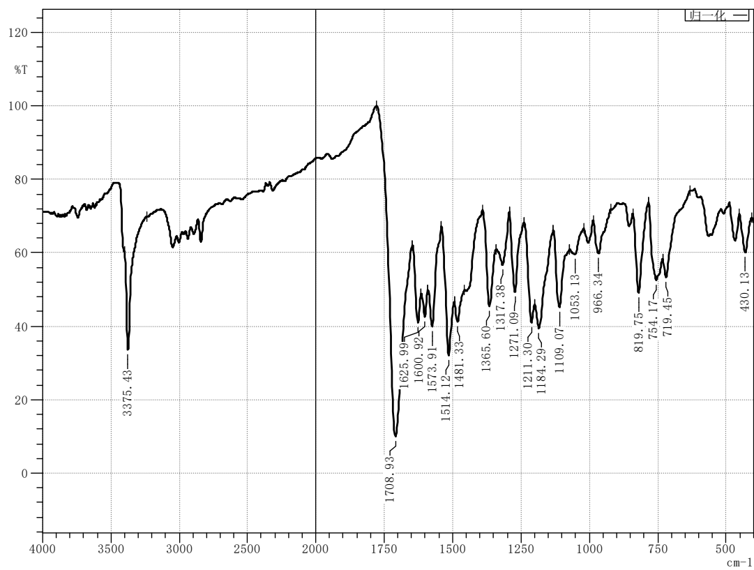
Figure 48 Infrared spectrum of compound M16
