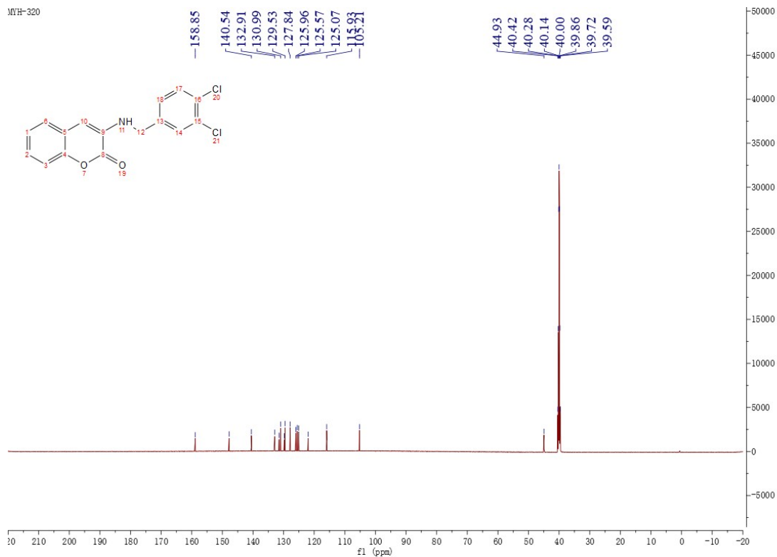
Figure 29 13 CNMR Spectrum of Compound M10
