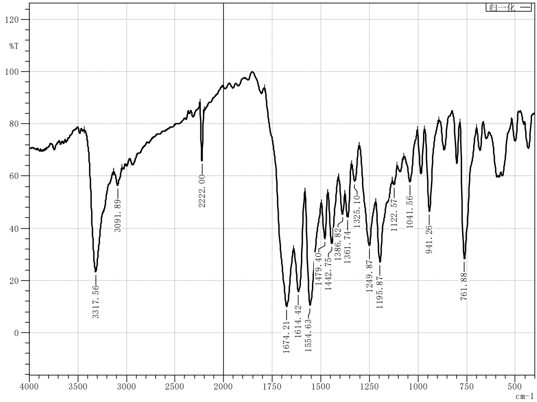
Figure 81 Infrared spectrum of compound M27
