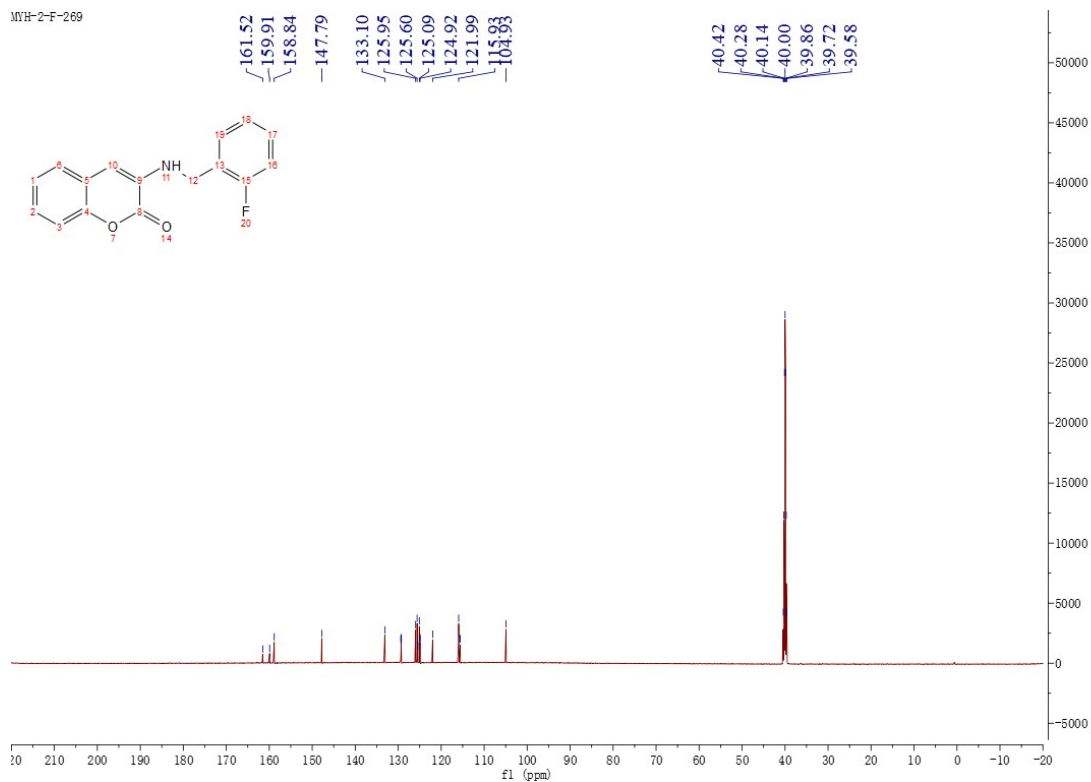
Figure 11 ^{13}\text{C} NMR Spectrum of Compound M4
