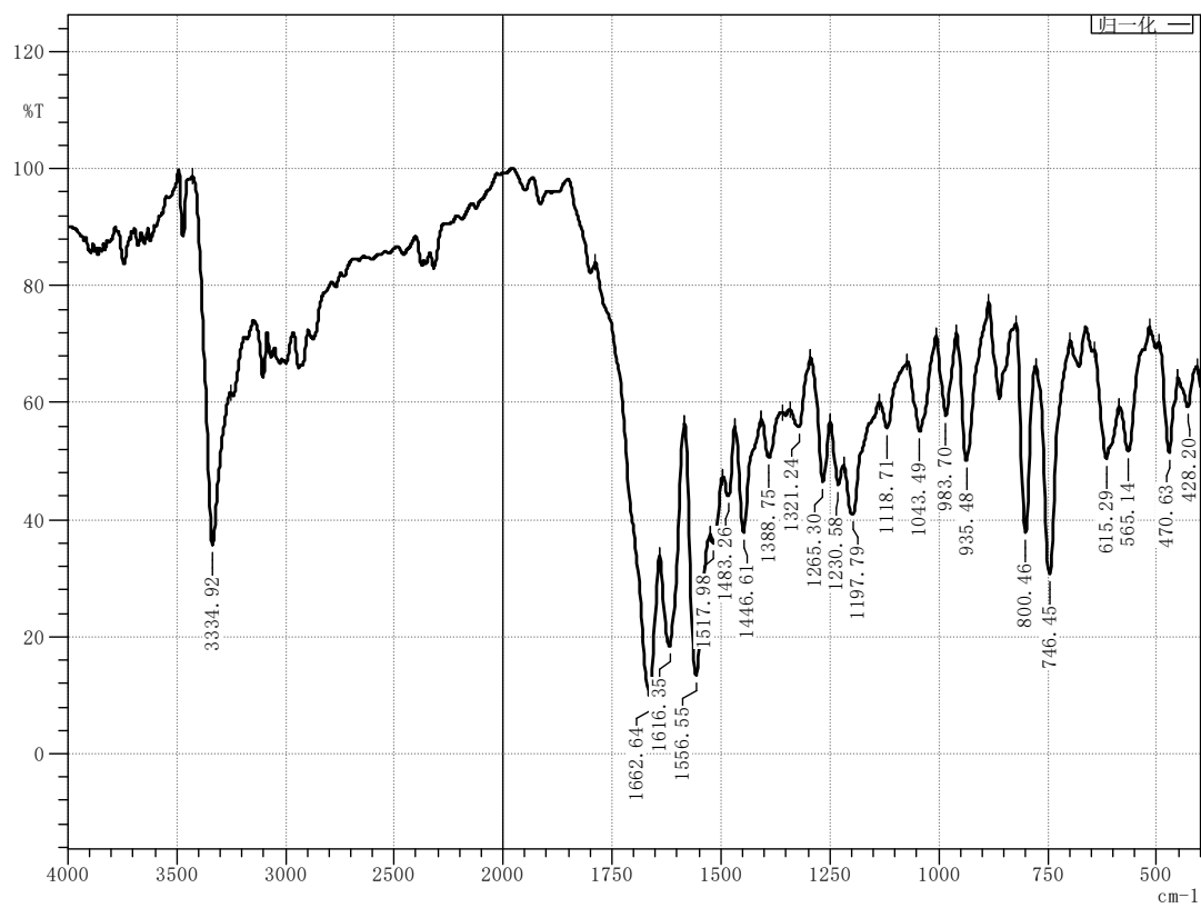
Figure 72 Infrared spectrum of compound M24
