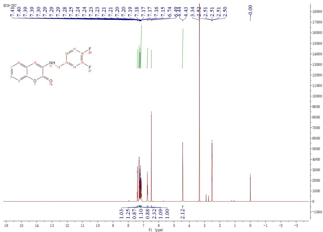
Figure 19 ^1\text{H NMR} Spectrum of Compound M7
