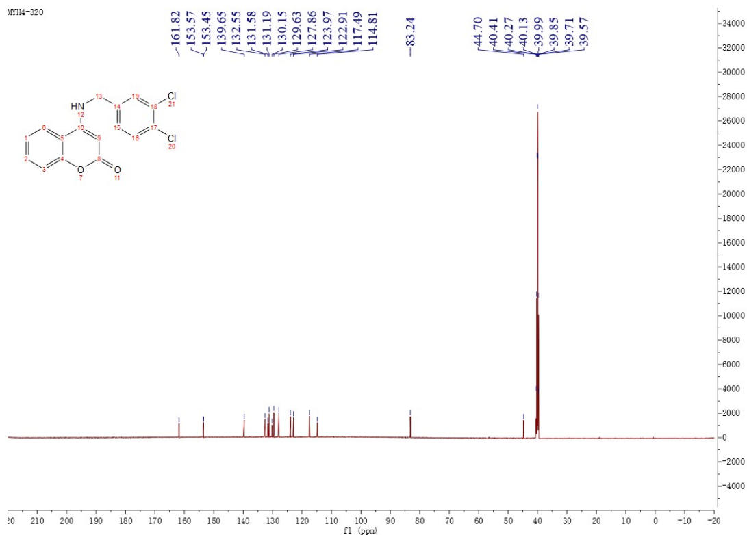
Figure 74 ^{13}\text{C} NMR Spectrum of Compound M25
