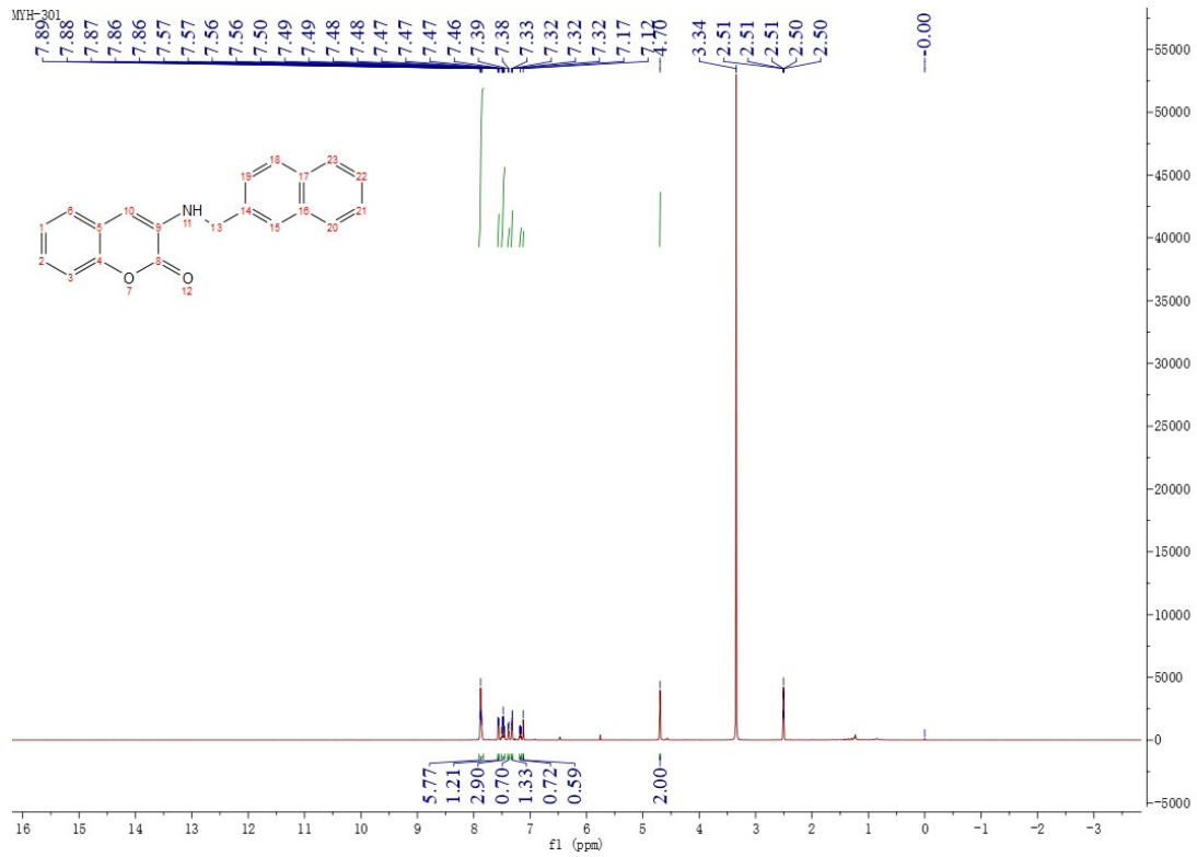
Figure 22 1 H NMR Spectrum of Compound M8
