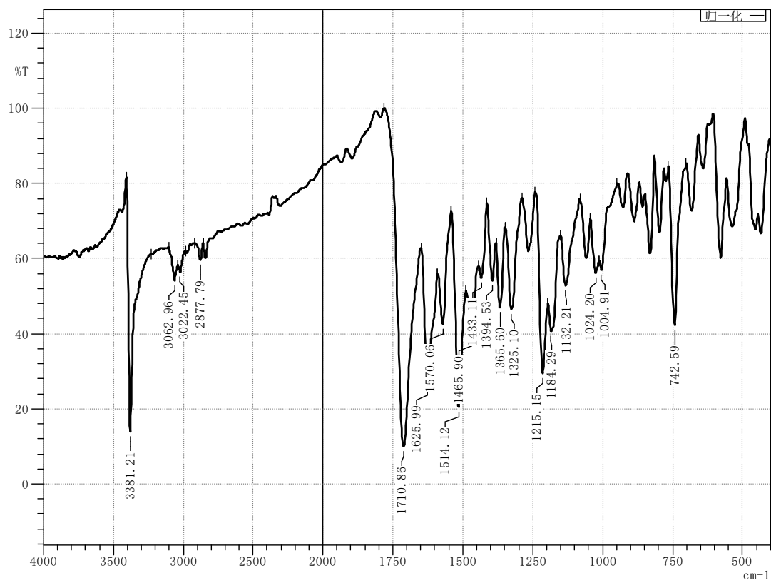
Figure 30 Infrared spectrum of compound M10
