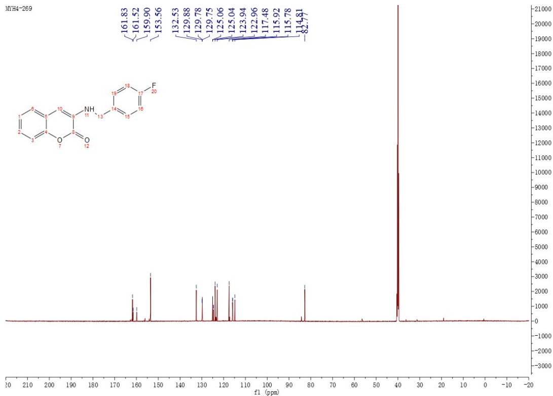
Figure 35 ^{13}\text{C} NMR Spectrum of Compound M12
