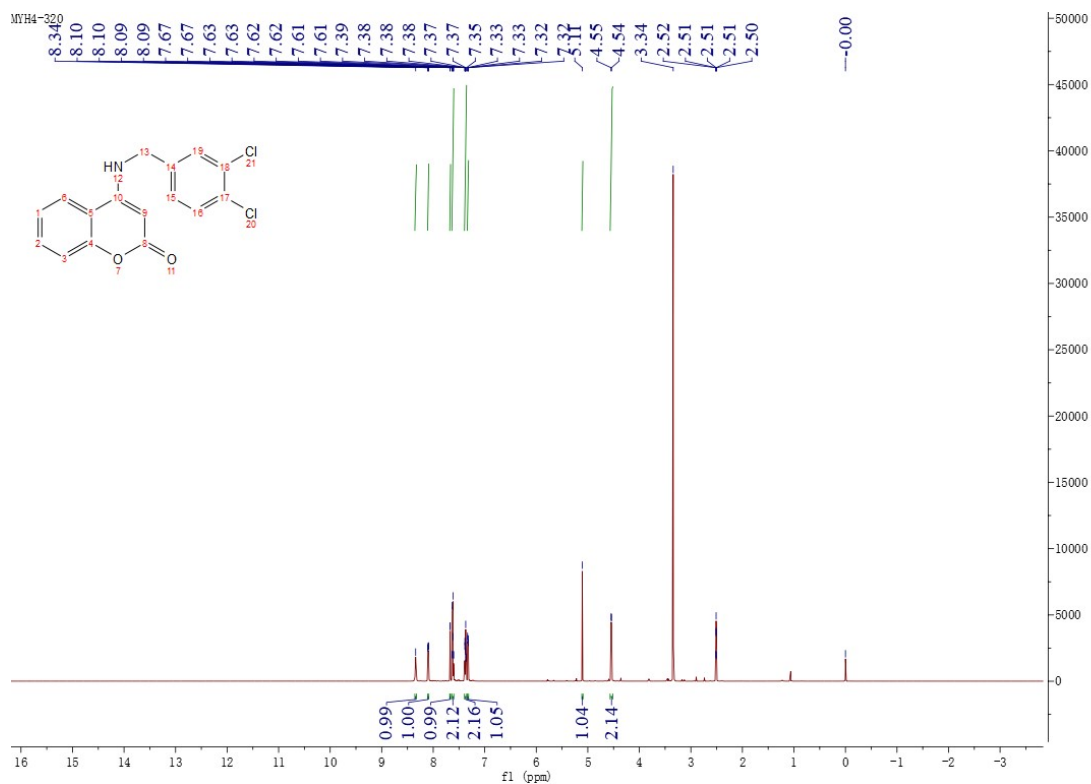
Figure 73 ^1\text{H} NMR Spectrum of Compound M25
