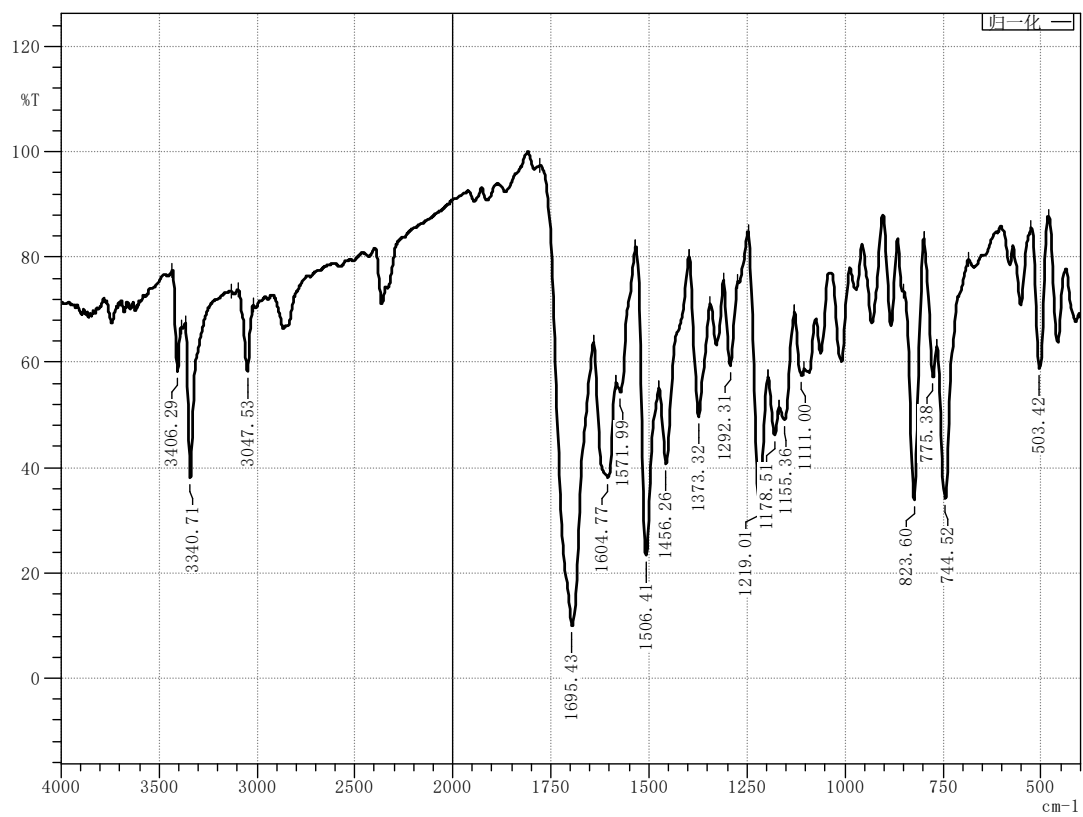
Figure 36 Infrared spectrum of compound M12
