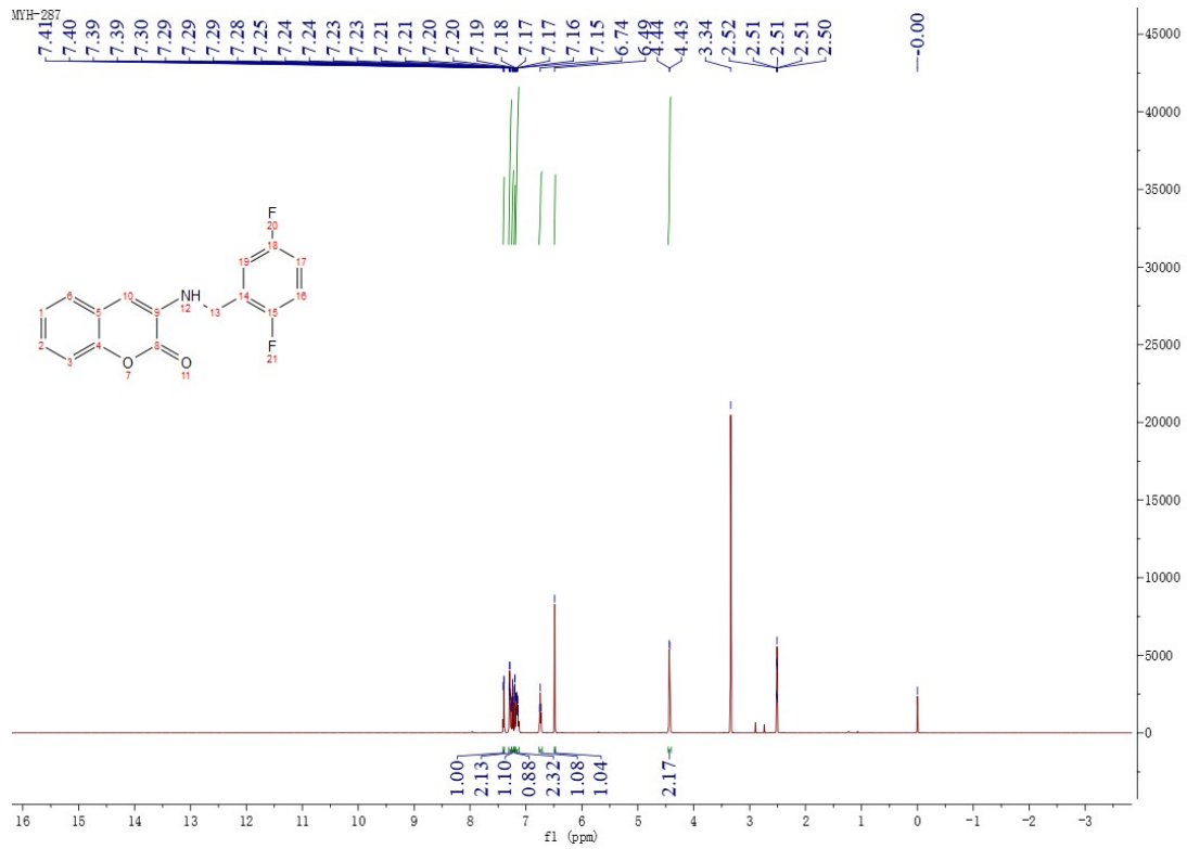
Figure 40 1 H NMR Spectrum of Compound M14
