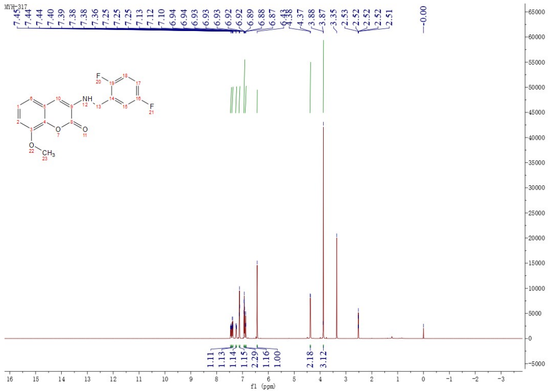
Figure 64 1 H NMR Spectrum of Compound M22
