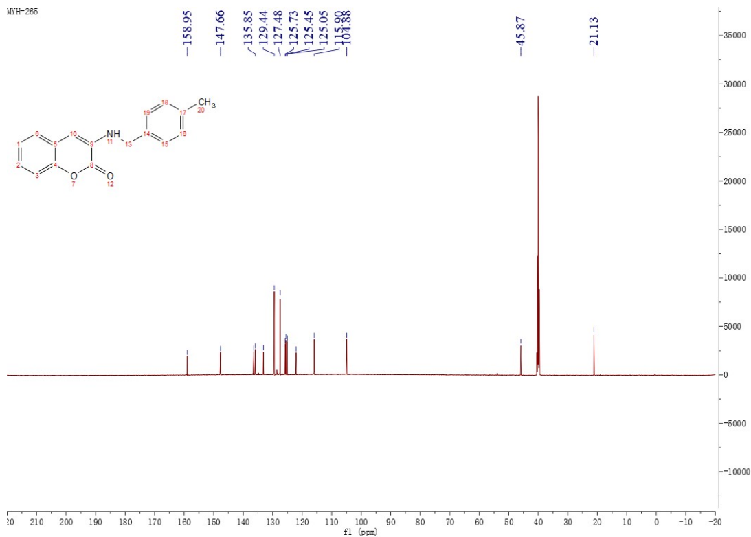
Figure 5 13 CNMR Spectrum of Compound M2
