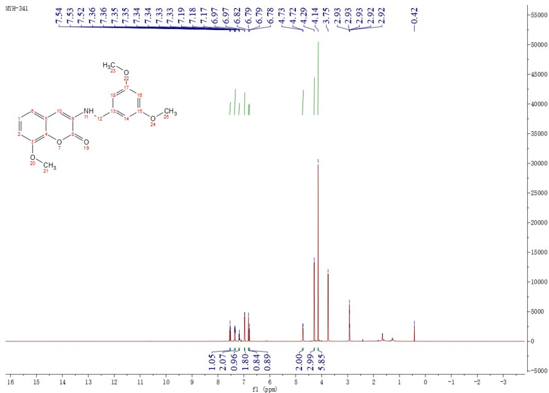
Figure 31 ^1\text{H} NMR Spectrum of Compound M11
