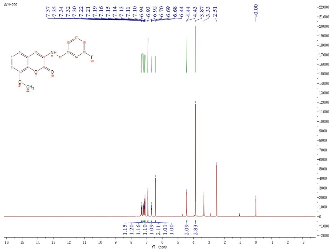
Figure 49 ^1\text{H NMR} Spectrum of Compound M17
