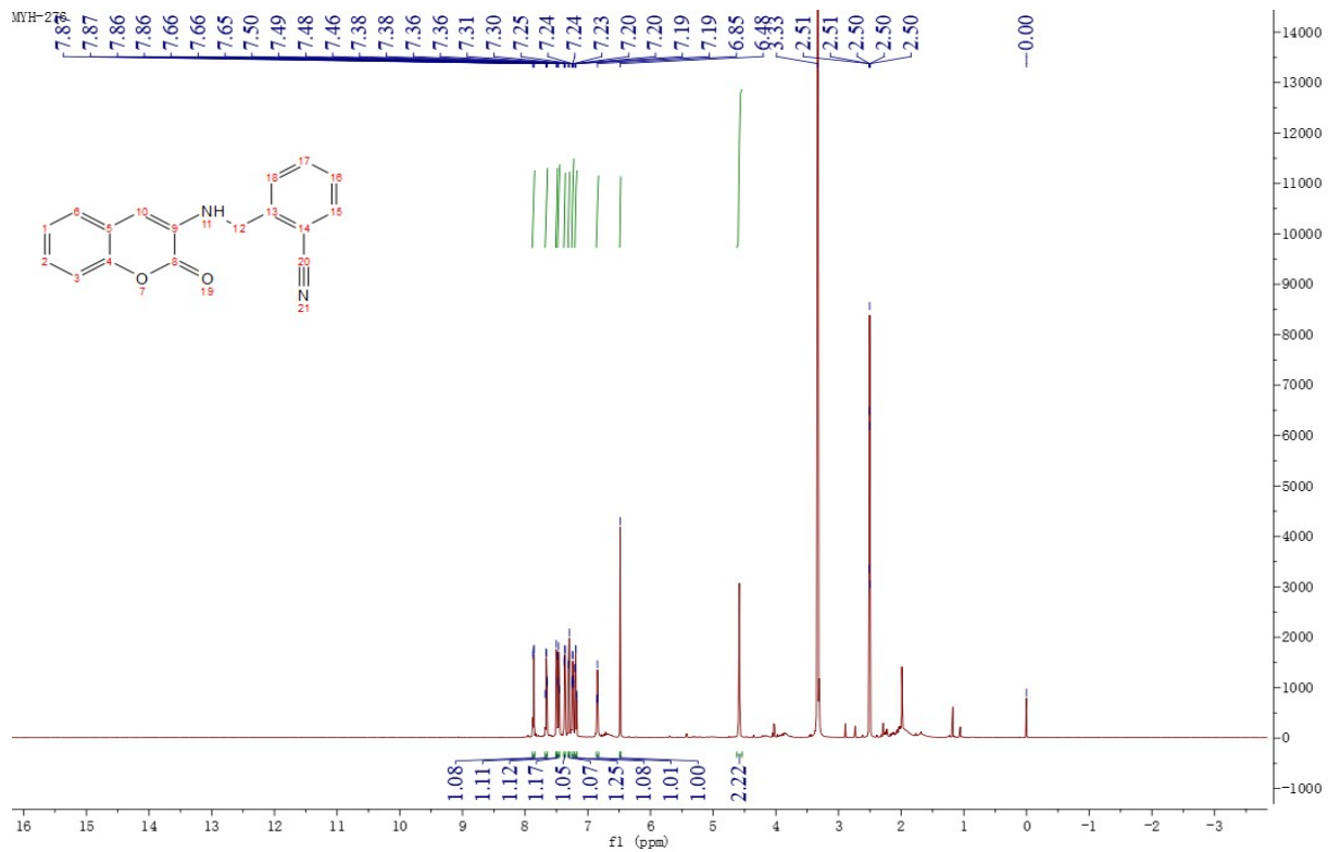
Figure 16 1 H NMR Spectrum of Compound M6
