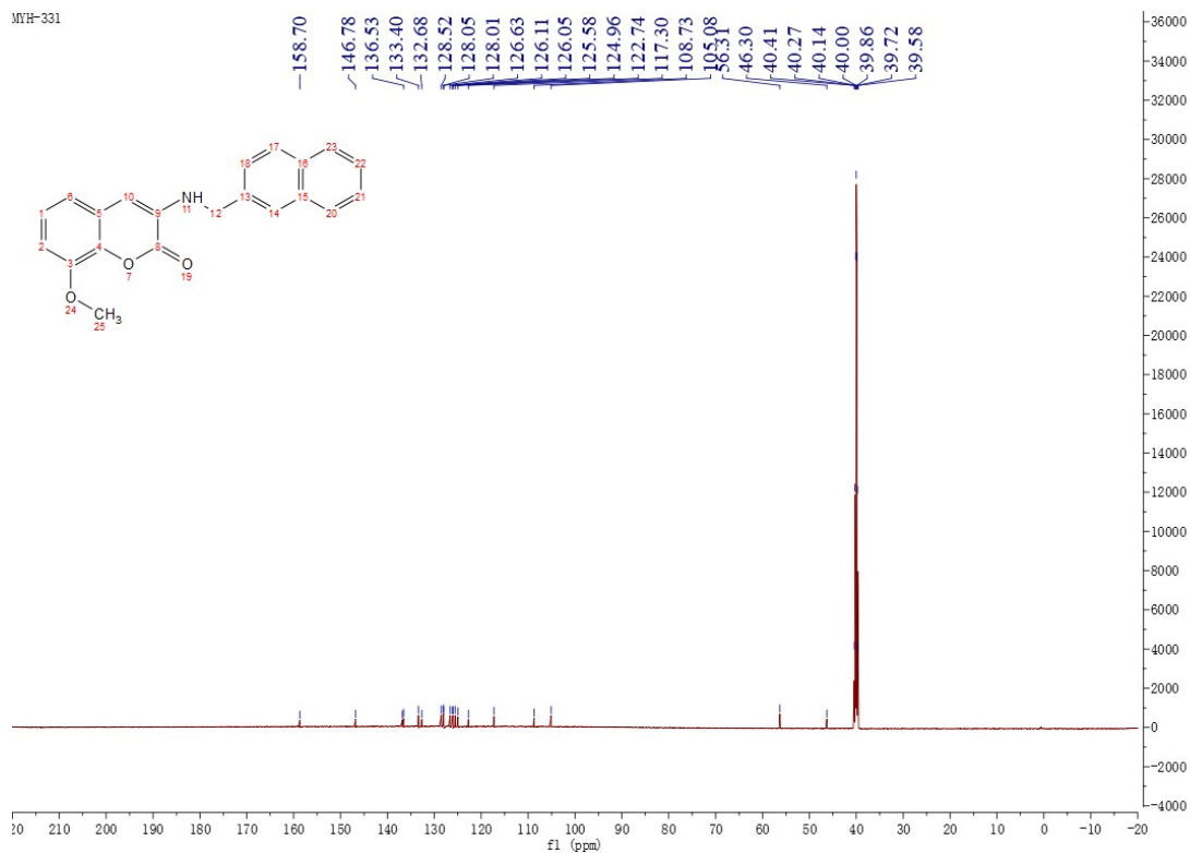
Figure 47 13 C NMR Spectrum of Compound M16
