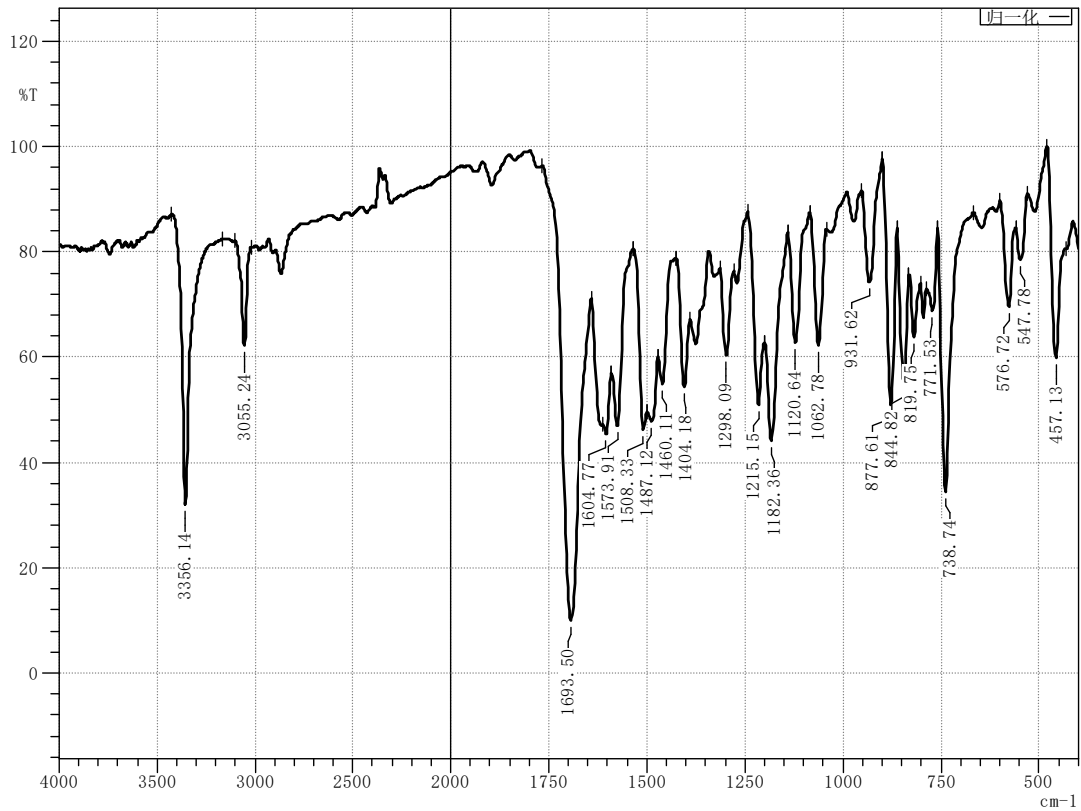
Figure 27 Infrared spectrum of compound M9
