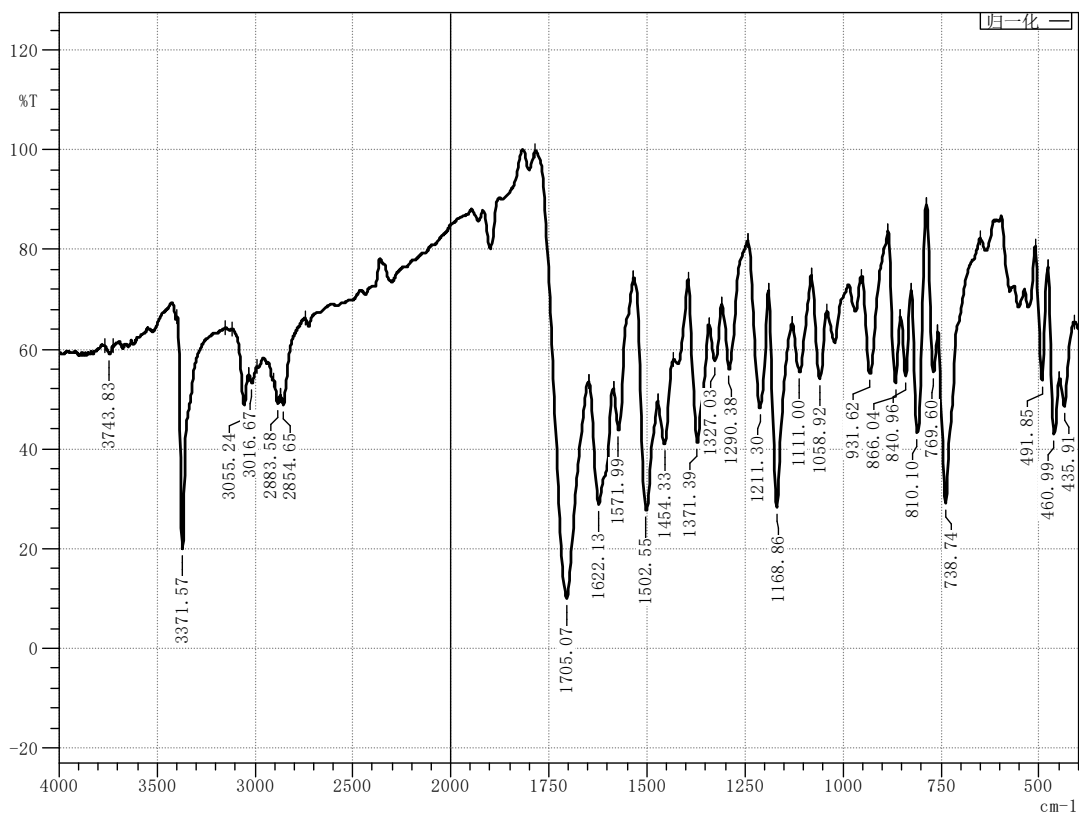
Figure 6 Infrared spectrum of compound M2
