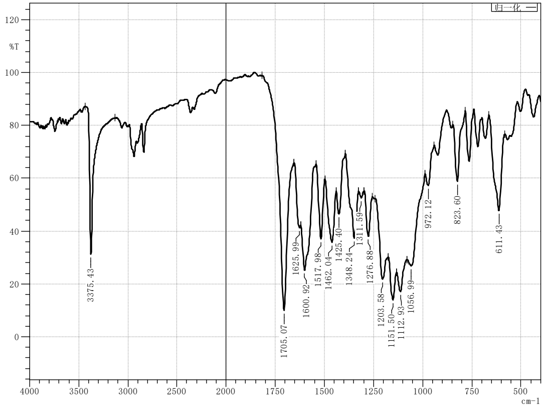
Figure 33 Infrared spectrum of compound M11
