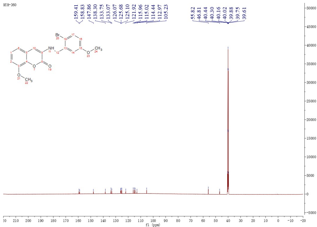
Figure 59 13 CNMR Spectrum of Compound M20
