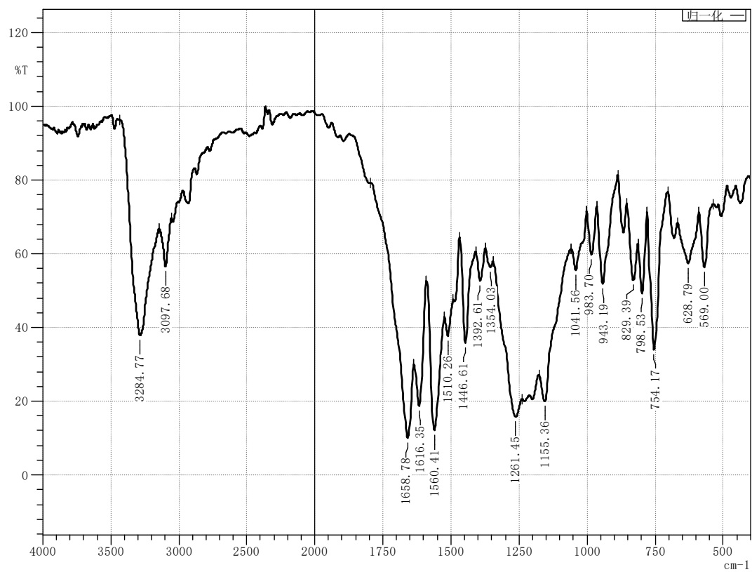
Figure 78 Infrared spectrum of compound M26
