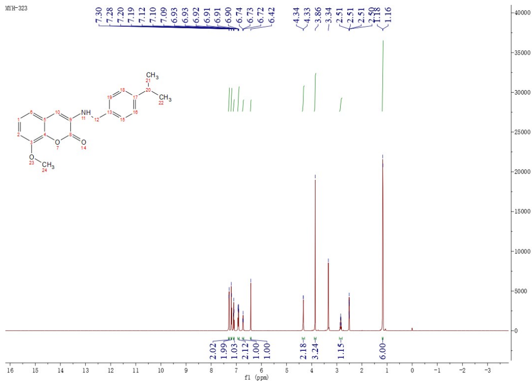
Figure 43 ^1\text{H NMR} Spectrum of Compound M15
