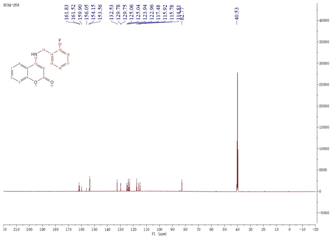
Figure 83 13 C NMR Spectrum of Compound M28
