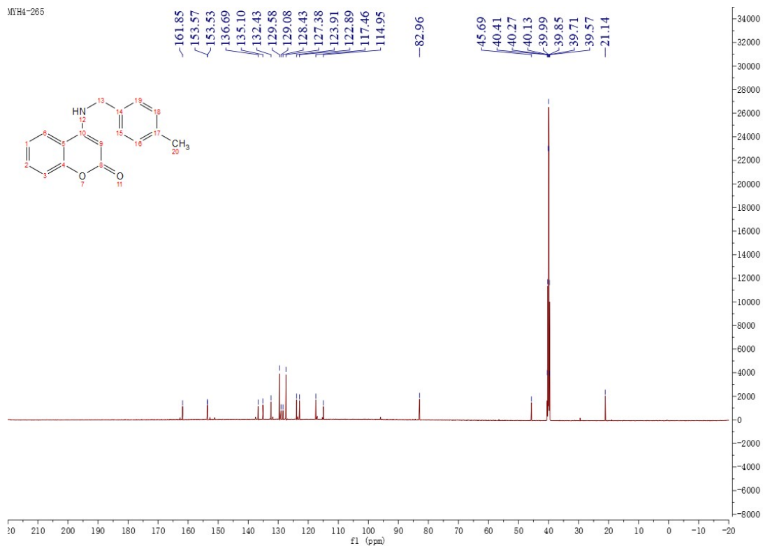
Figure 71 13 CNMR Spectrum of Compound M24
