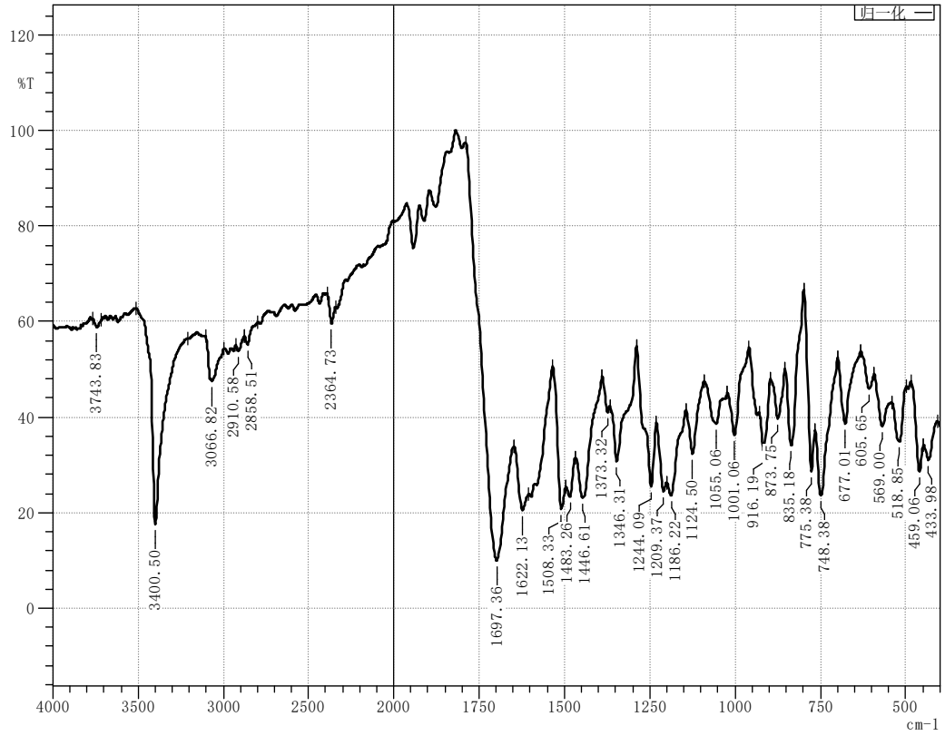
Figure 15 Infrared spectrum of compound M5
