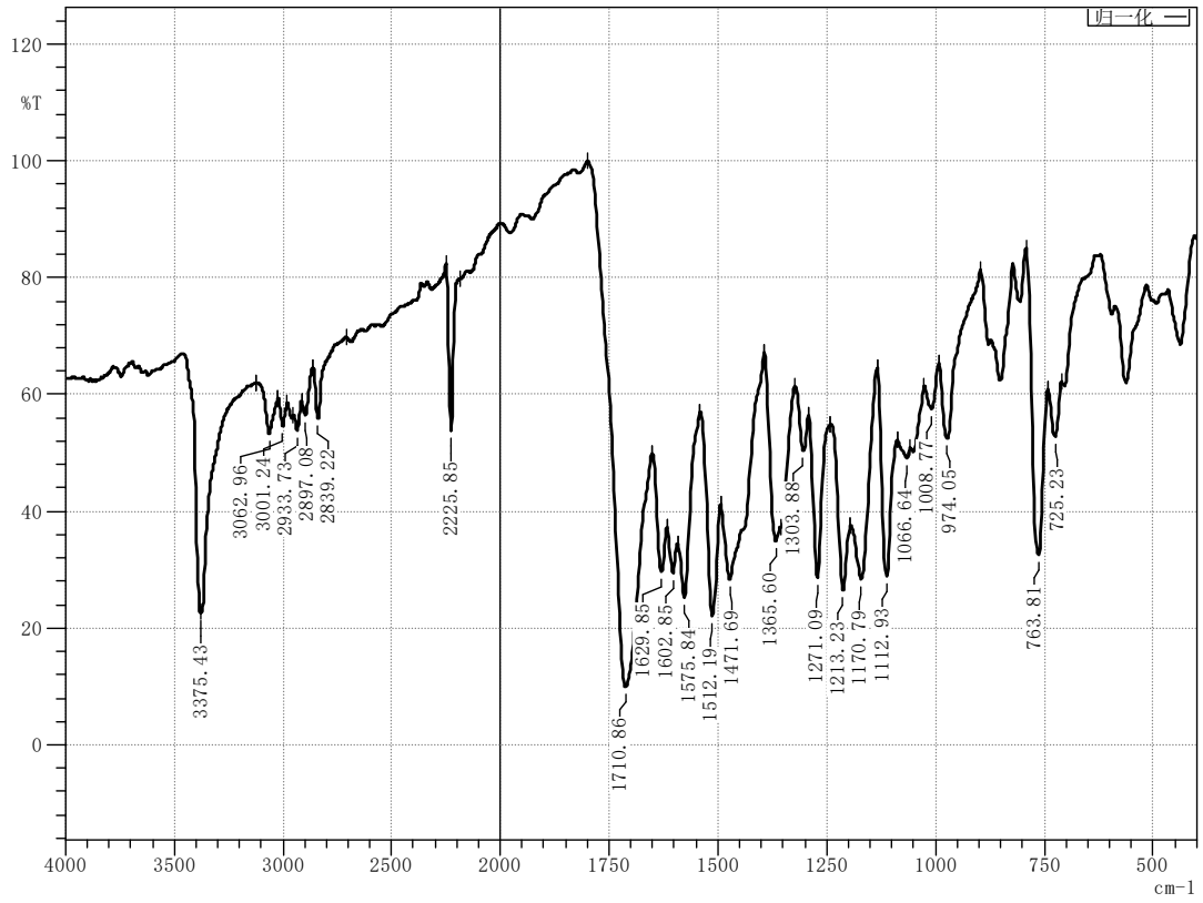
Figure 69 Infrared spectrum of compound M23
