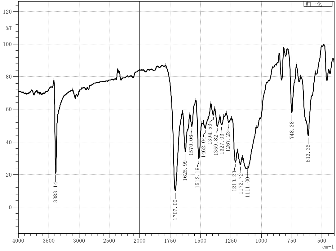
Figure 3 Infrared spectrum of compound M1
