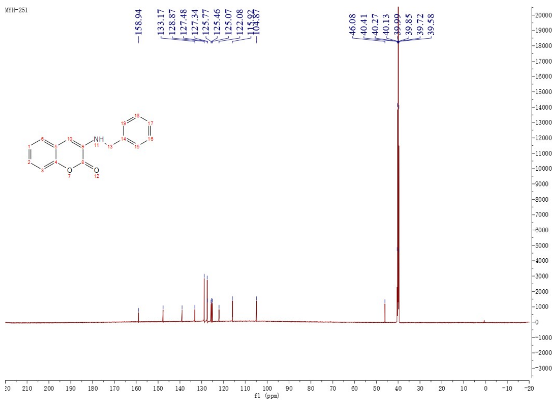
Figure 2 13 C NMR Spectrum of Compound M1
