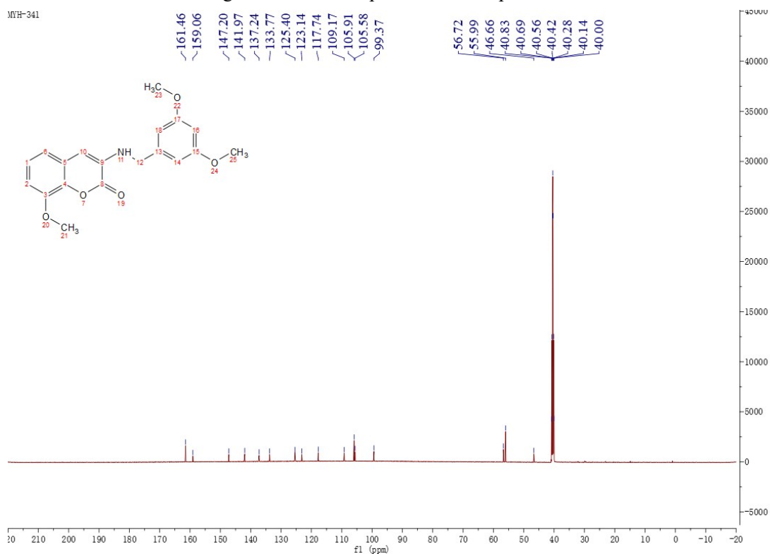
Figure 32 ^{13}\text{C} NMR Spectrum of Compound M11
