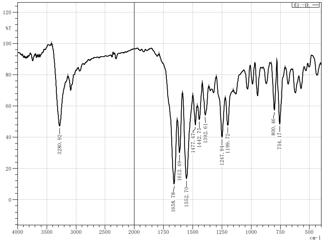
Figure 75 Infrared spectrum of compound M25
