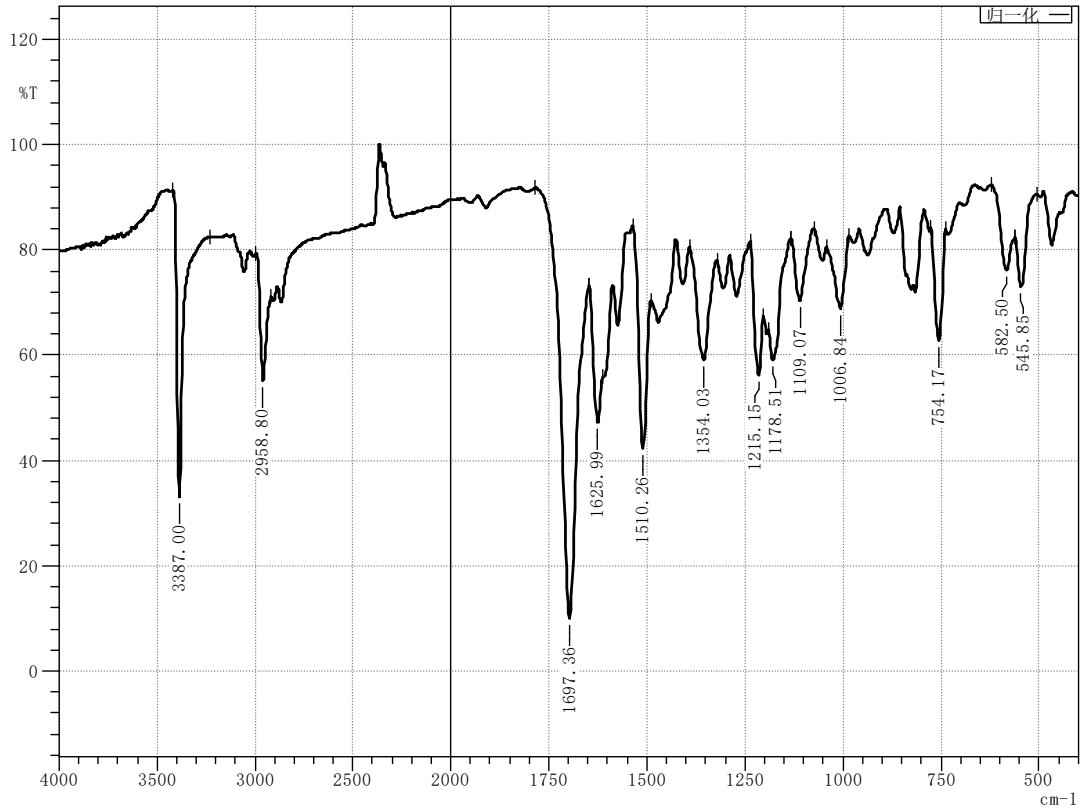
Figure 39 Infrared spectrum of compound M13
