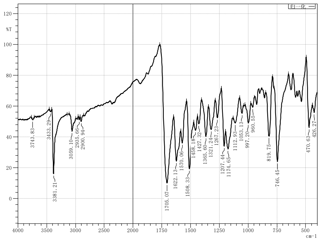
Figure 24 Infrared spectrum of compound M8
