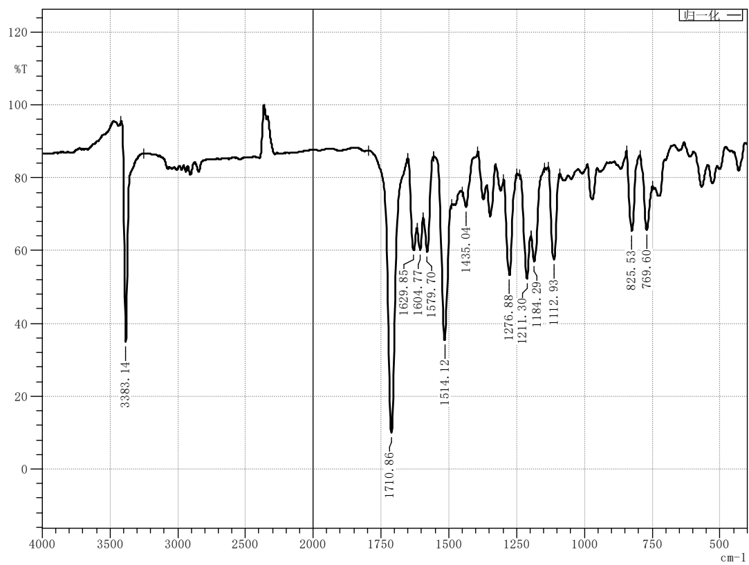
Figure 66 Infrared spectrum of compound M22
