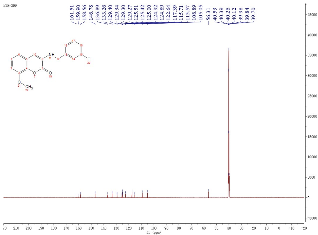
Figure 50 ^{13}\text{C NMR} Spectrum of Compound M17
