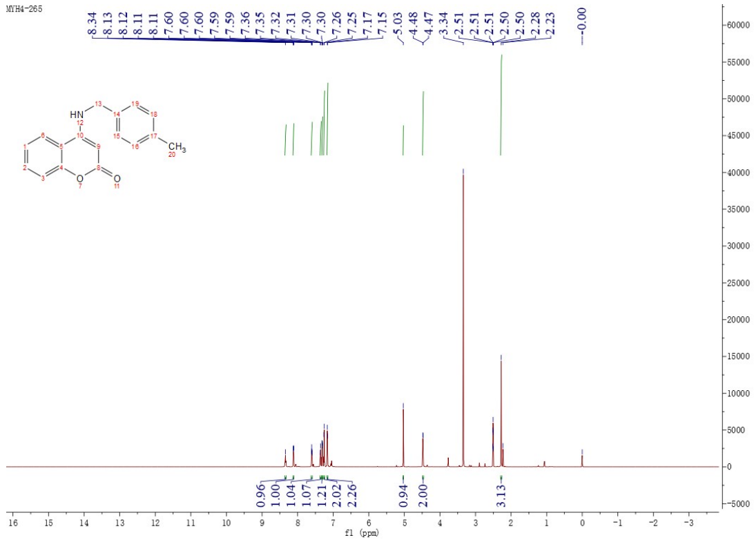
Figure 70 1 H NMR Spectrum of Compound M24
