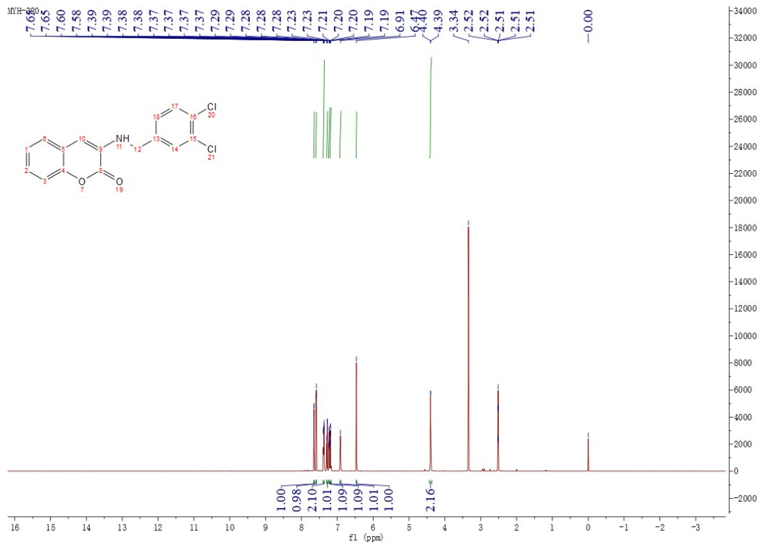
Figure 28 1 H NMR Spectrum of Compound M10
