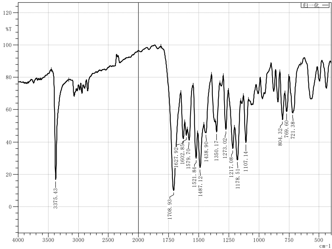
Figure 57 Infrared spectrum of compound M19
