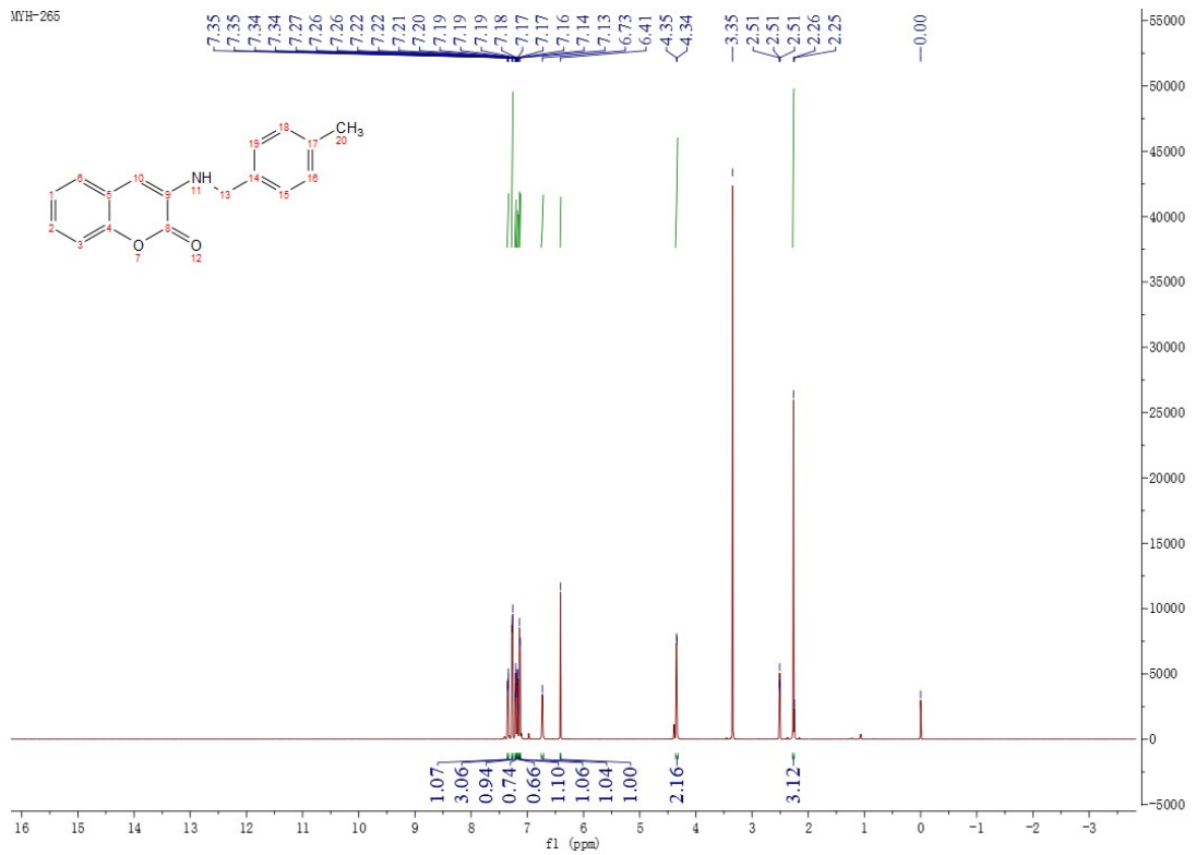
Figure 4 1 H NMR Spectrum of Compound M2
