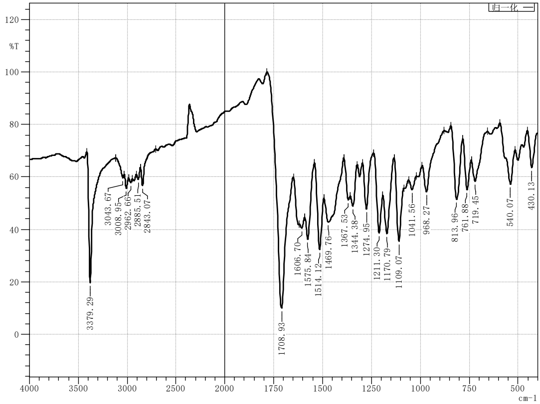
Figure 63 Infrared spectrum of compound M21
