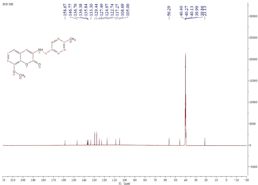
Figure 62 13 C NMR Spectrum of Compound M21
