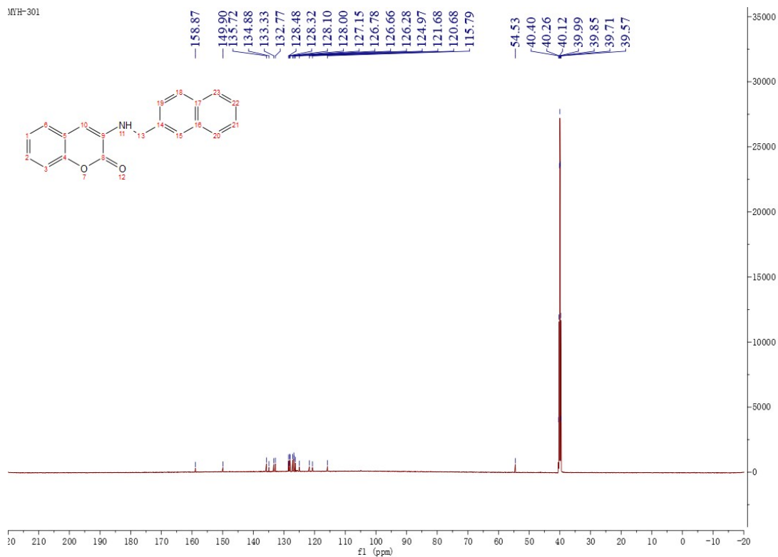
Figure 23 13 C NMR Spectrum of Compound M8
