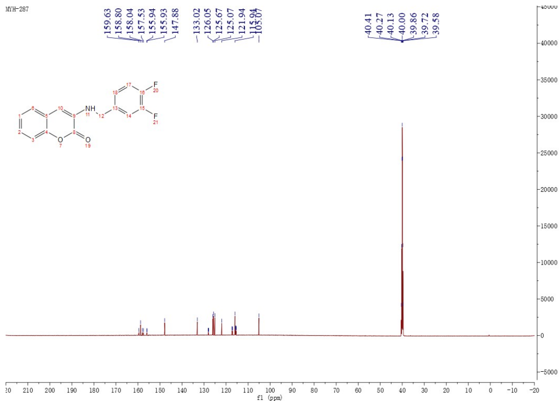
Figure 20 ^{13}\text{C NMR} Spectrum of Compound M7
