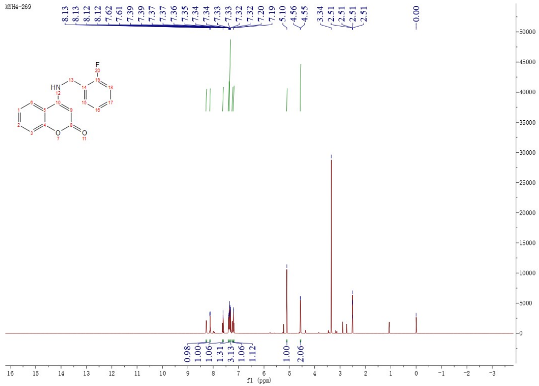
Figure 82 1 H NMR Spectrum of Compound M28
