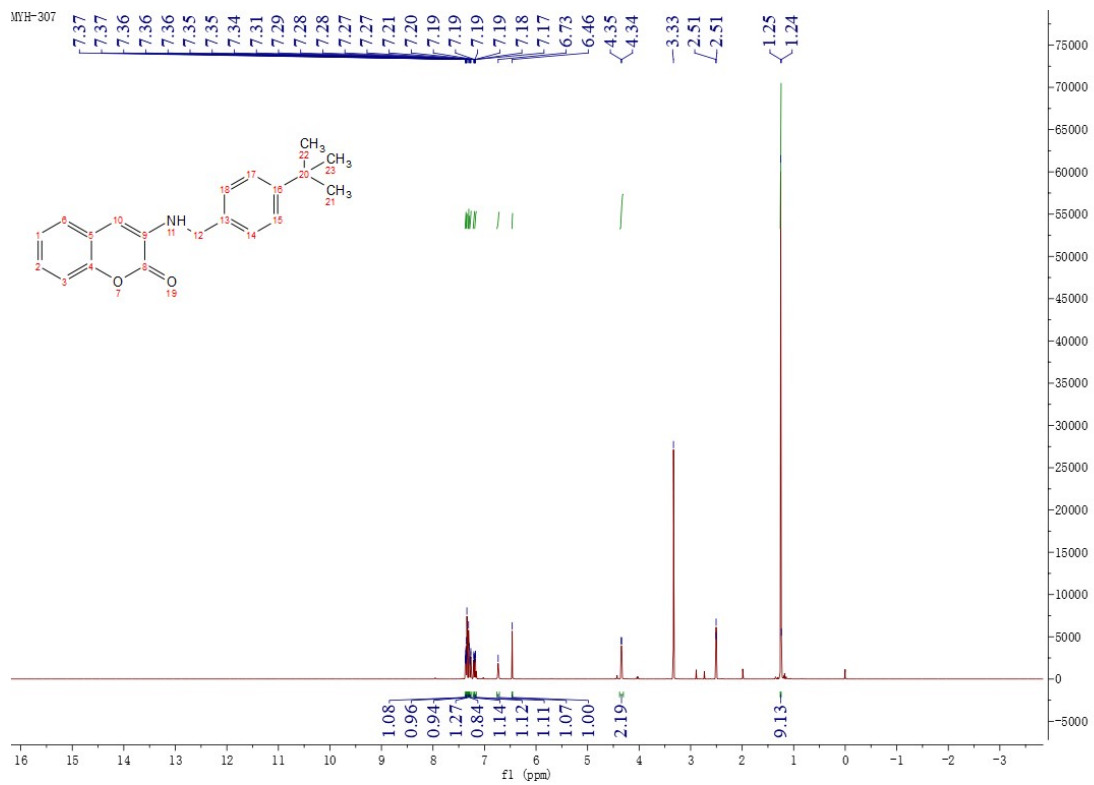
Figure 37 1 H NMR Spectrum of Compound M13
