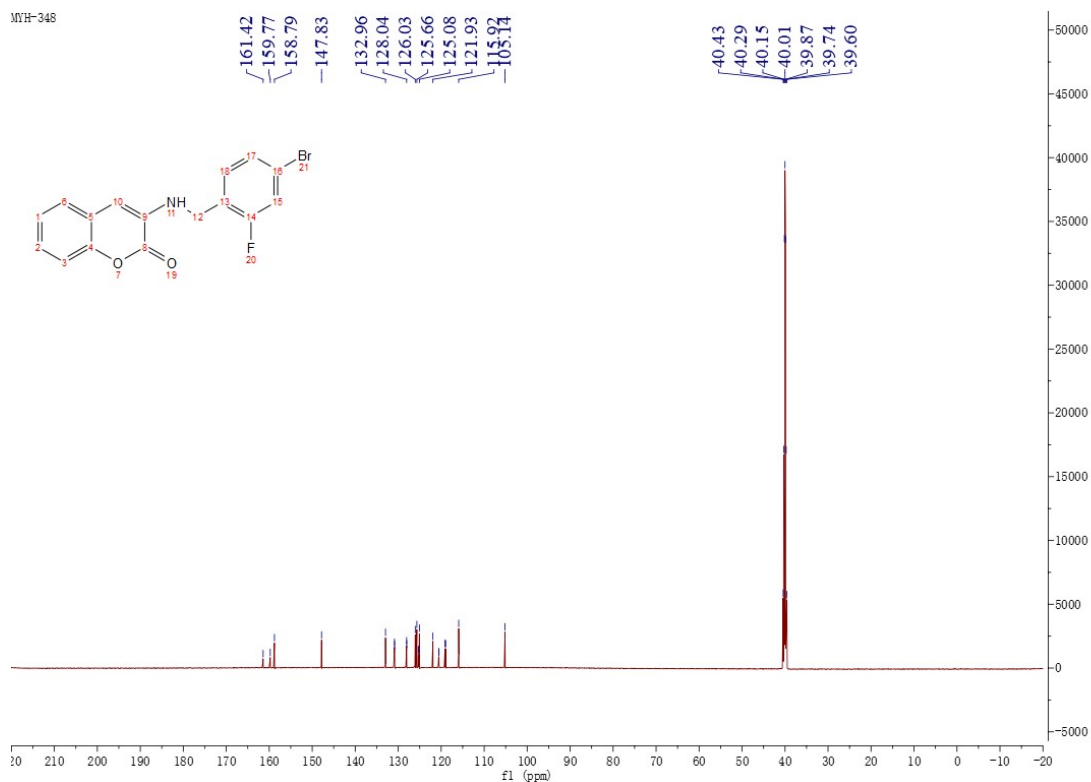
Figure 26 ^{13}\text{C NMR} Spectrum of Compound M9
