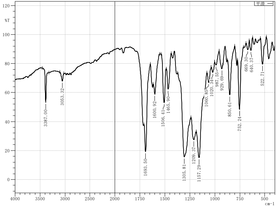
Figure 9 Infrared spectrum of compound M3
