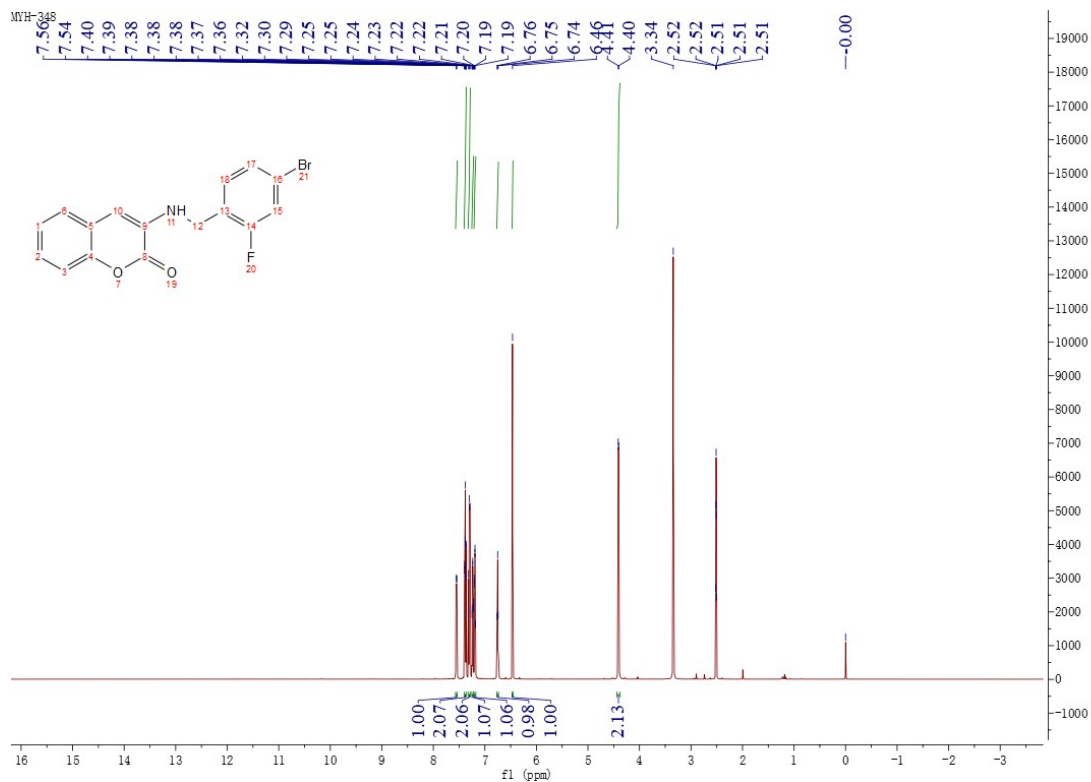
Figure 25 ^1\text{H NMR} Spectrum of Compound M9
