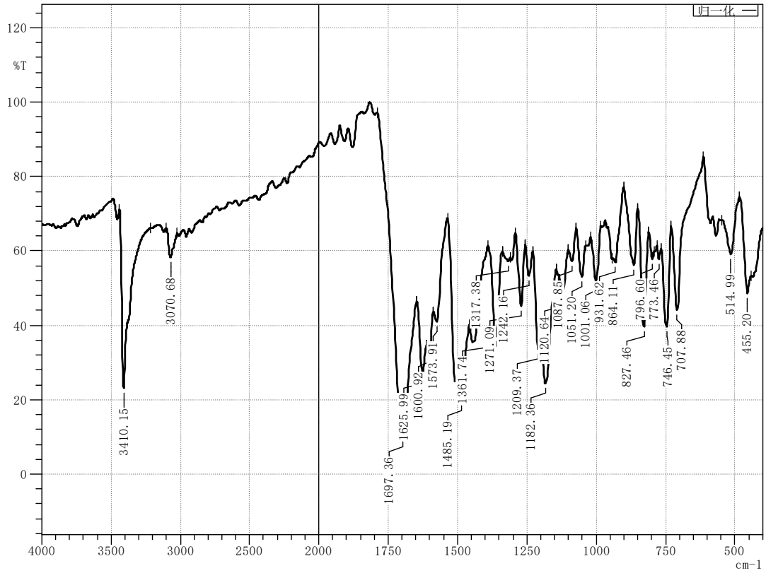
Figure 21 Infrared spectrum of compound M7
