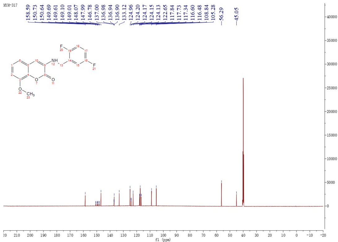
Figure 65 13 C NMR Spectrum of Compound M22
