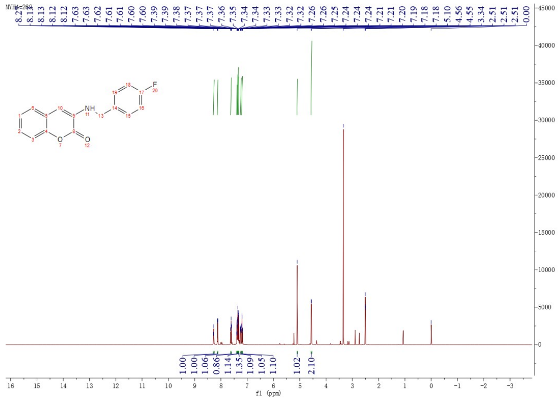
Figure 34 1 H NMR Spectrum of Compound M12
