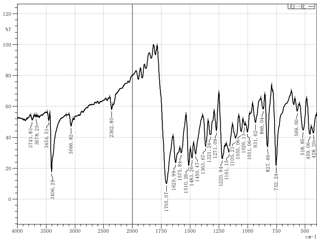
Figure 12 Infrared spectrum of compound M4
