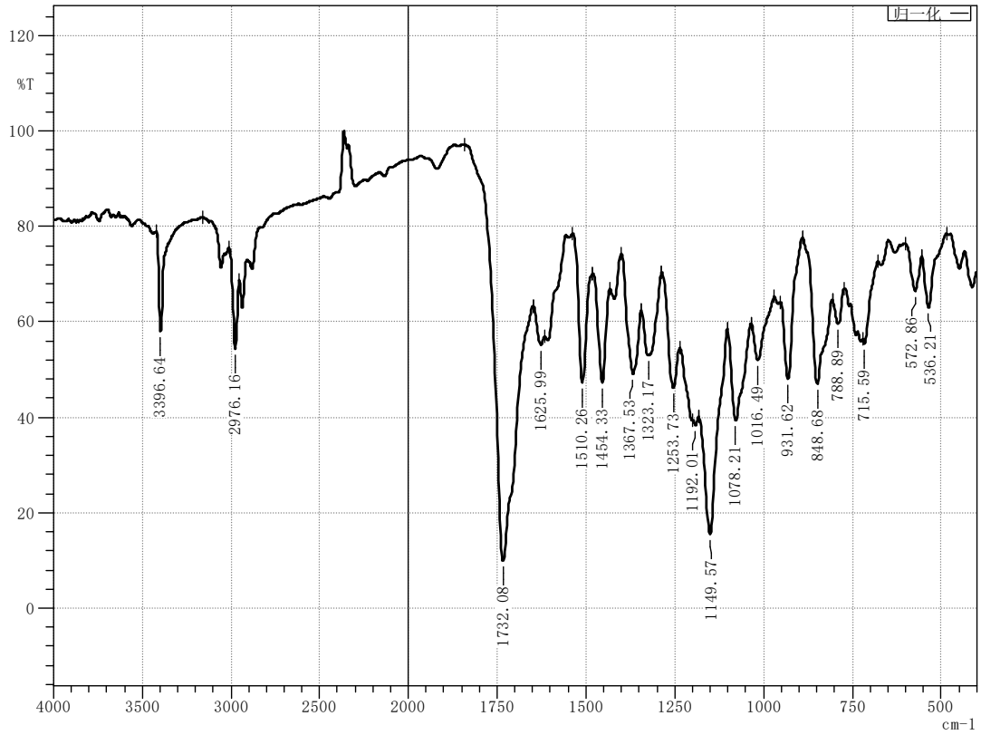
Figure 45 Infrared spectrum of compound M15
