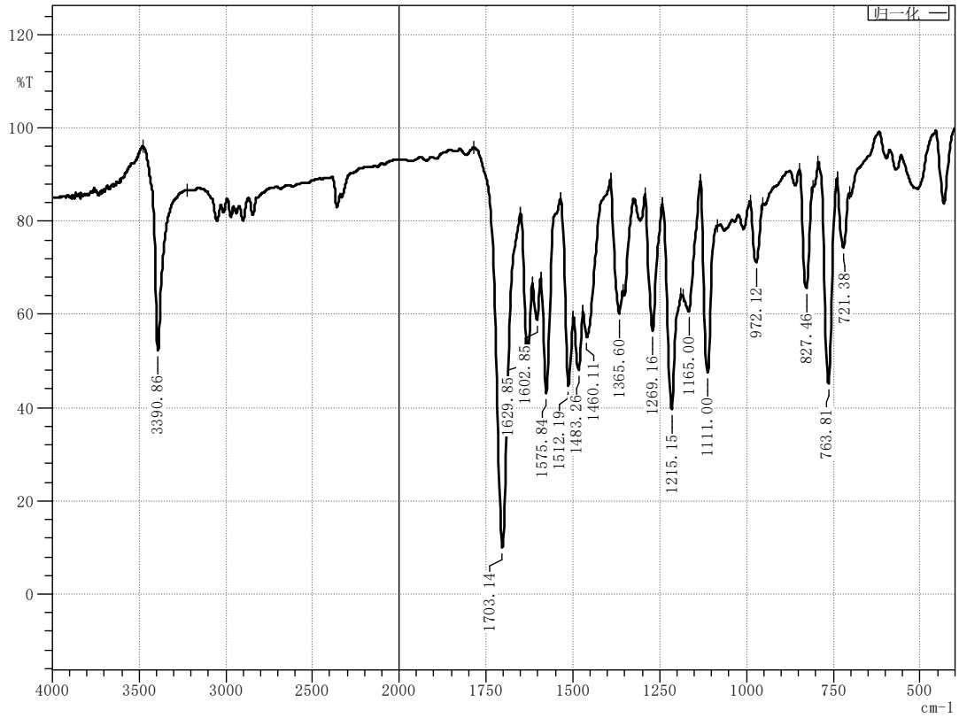
Figure 51 Infrared spectrum of compound M17
