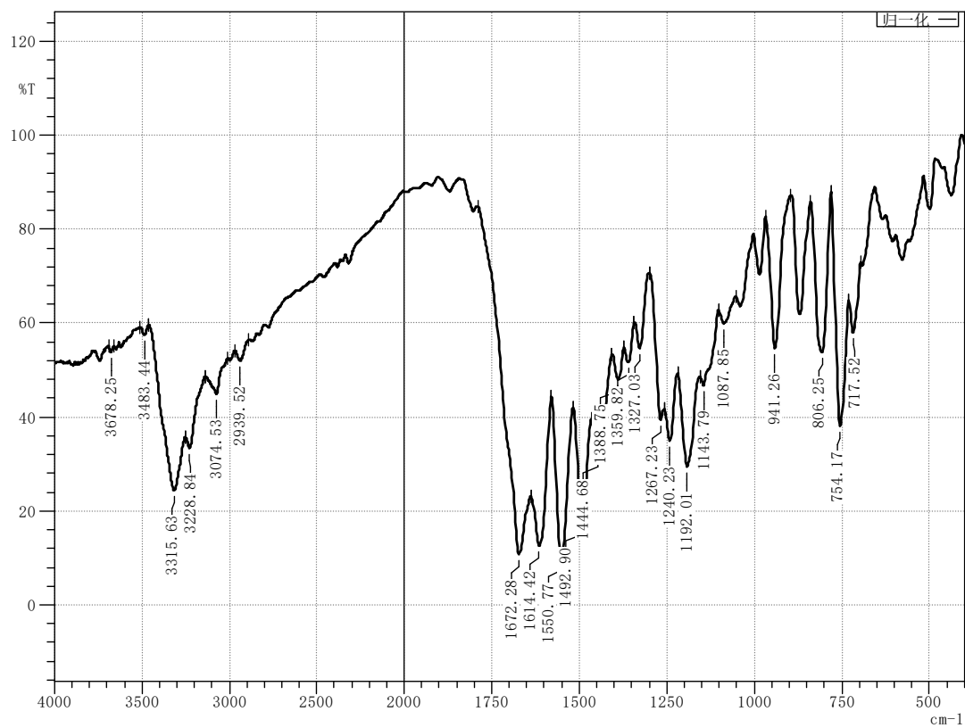
Figure 87 Infrared spectrum of compound M29
