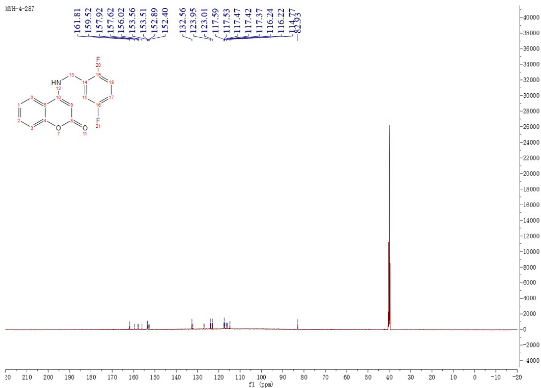
Figure 86 13 C NMR Spectrum of Compound M29
