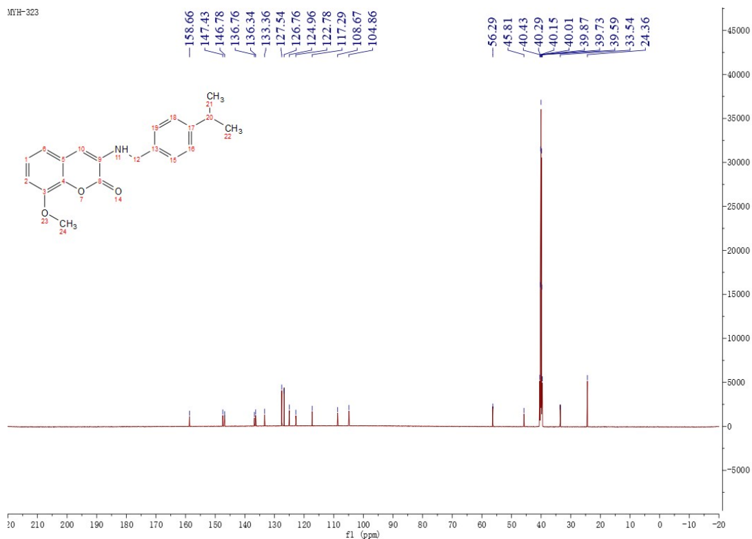
Figure 44 ^{13}\text{C NMR} Spectrum of Compound M15
