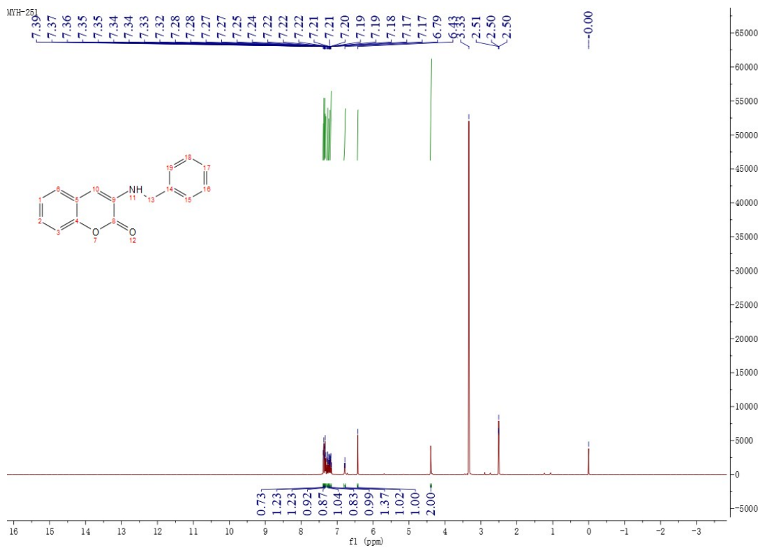
Figure 1 1 H NMR Spectrum of Compound M1
