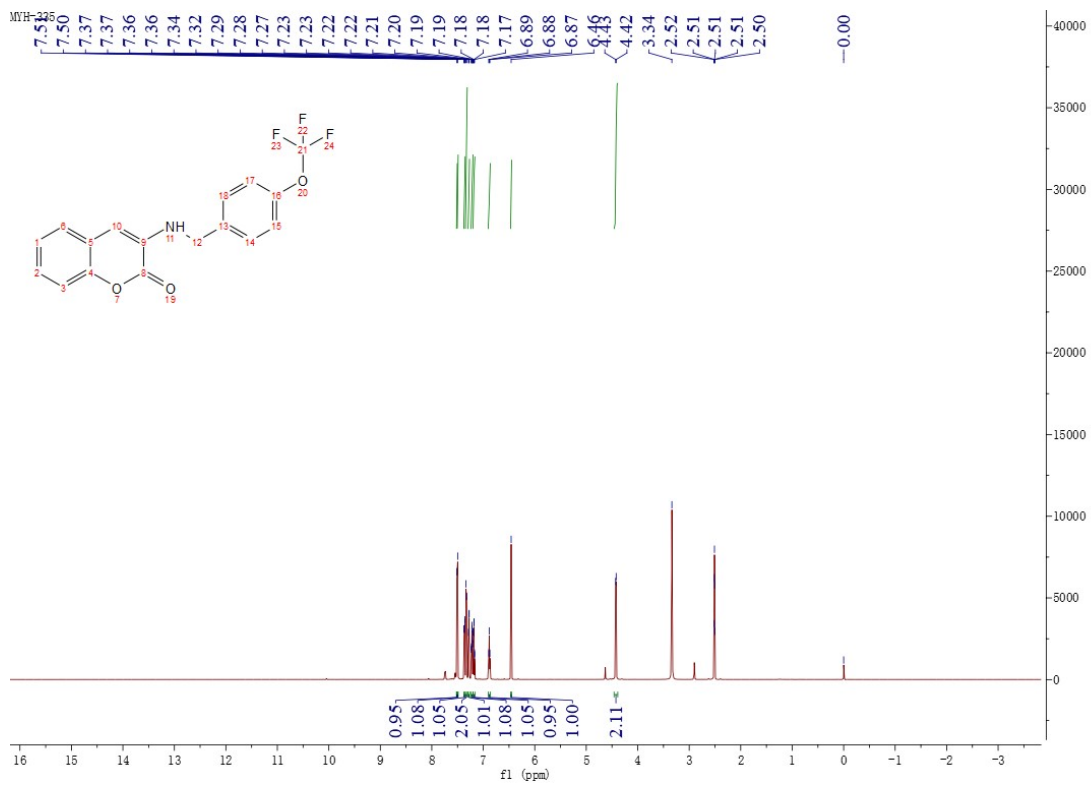
Figure 7 1 H NMR Spectrum of Compound M3
