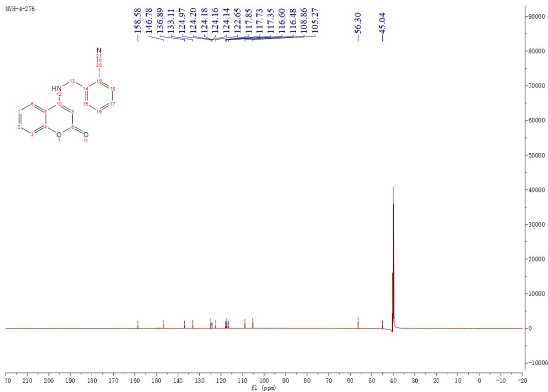
Figure 80 ^{13}\text{C NMR} Spectrum of Compound M27
