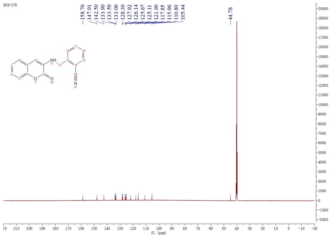
Figure 17 13 C NMR Spectrum of Compound M17
