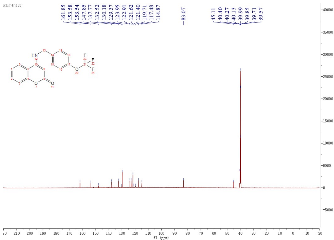
Figure 77 13 CNMR Spectrum of Compound M26
