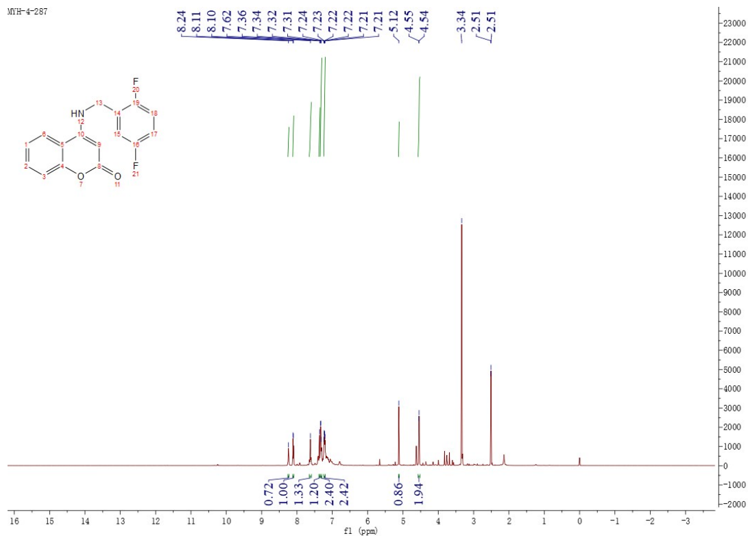
Figure 85 1 H NMR Spectrum of Compound M29
