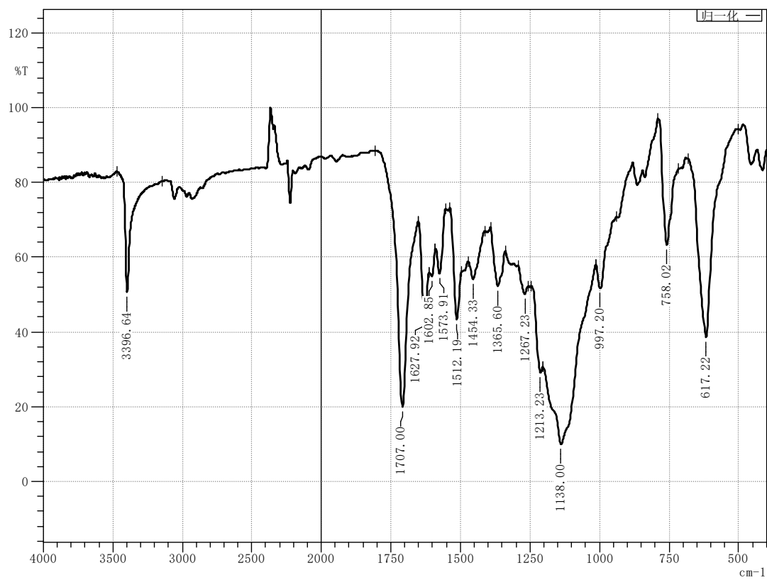
Figure 18 Infrared spectrum of compound M6
