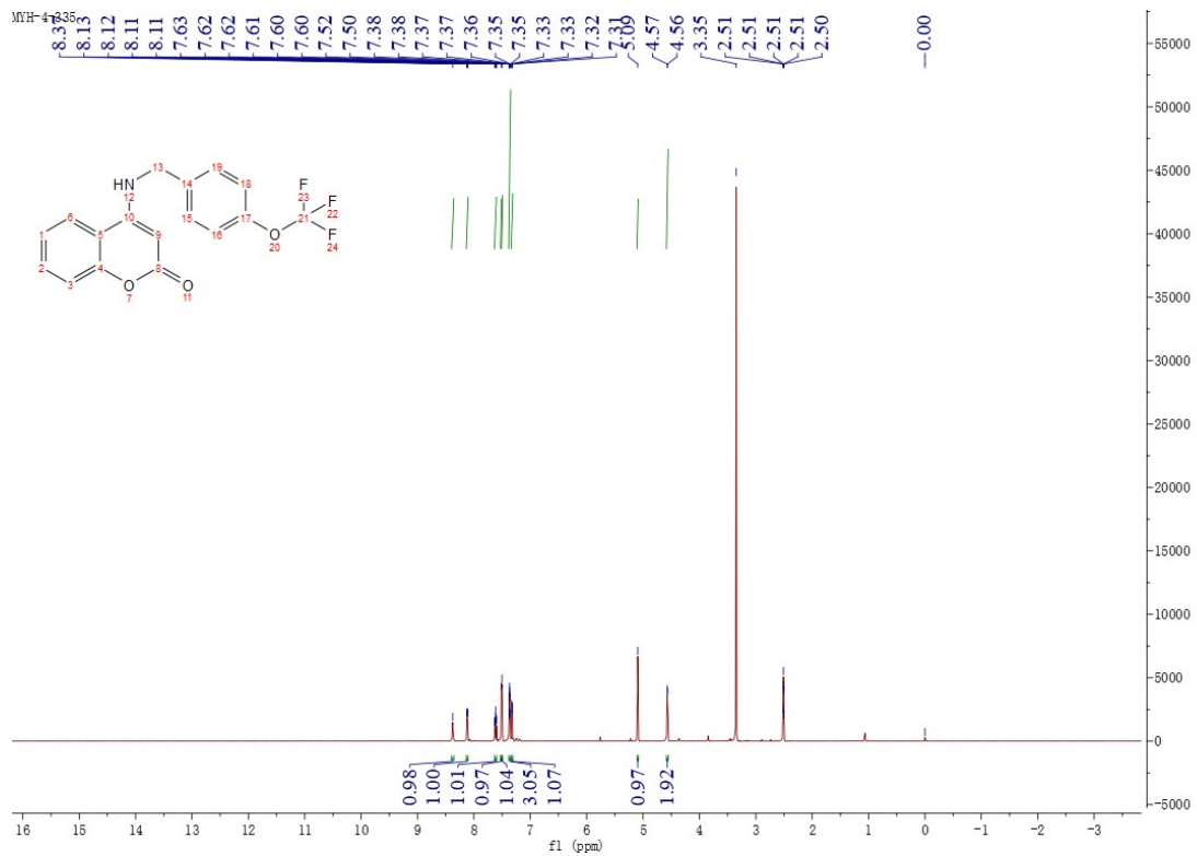
Figure 76 1 H NMR Spectrum of Compound M26
