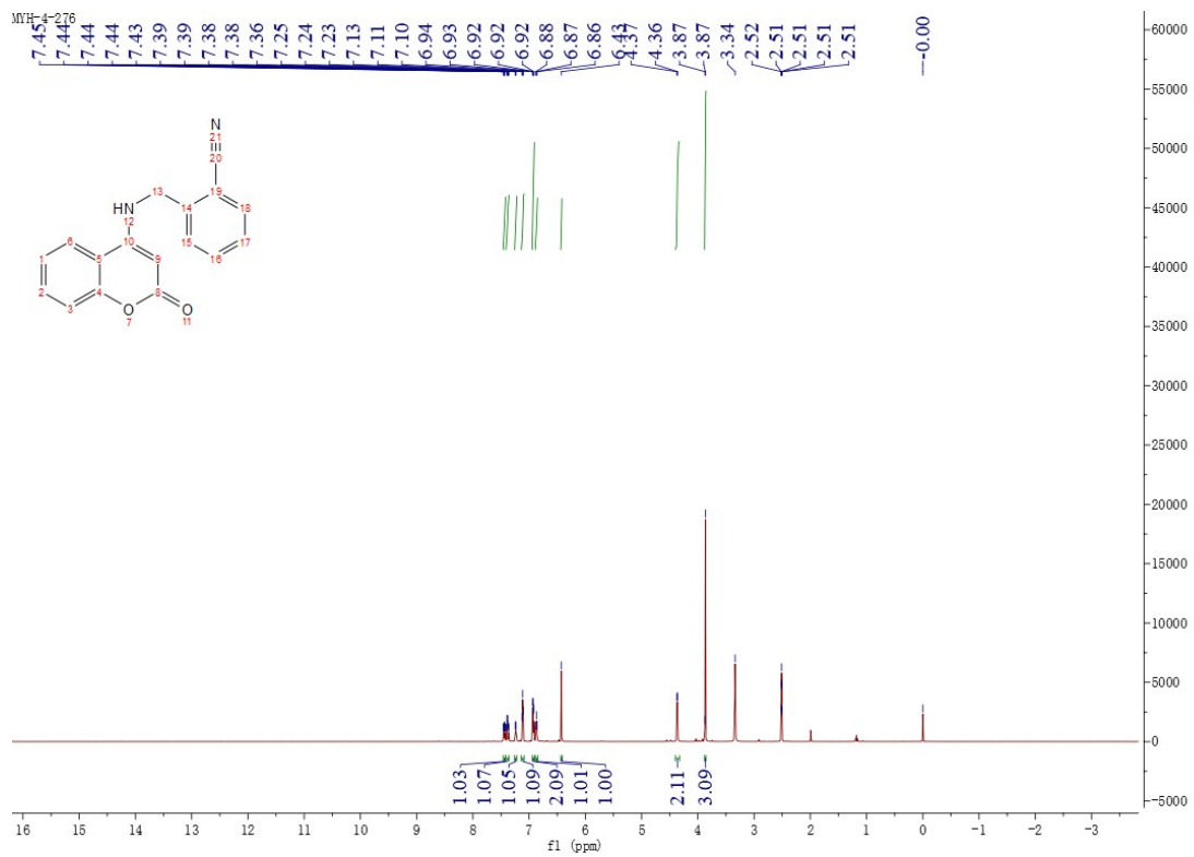
Figure 79 ^1\text{H NMR} Spectrum of Compound M27
