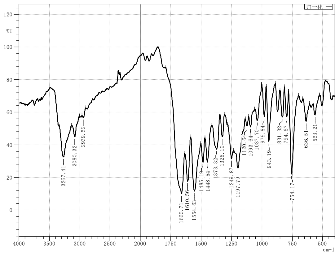
Figure 84 Infrared spectrum of compound M28
