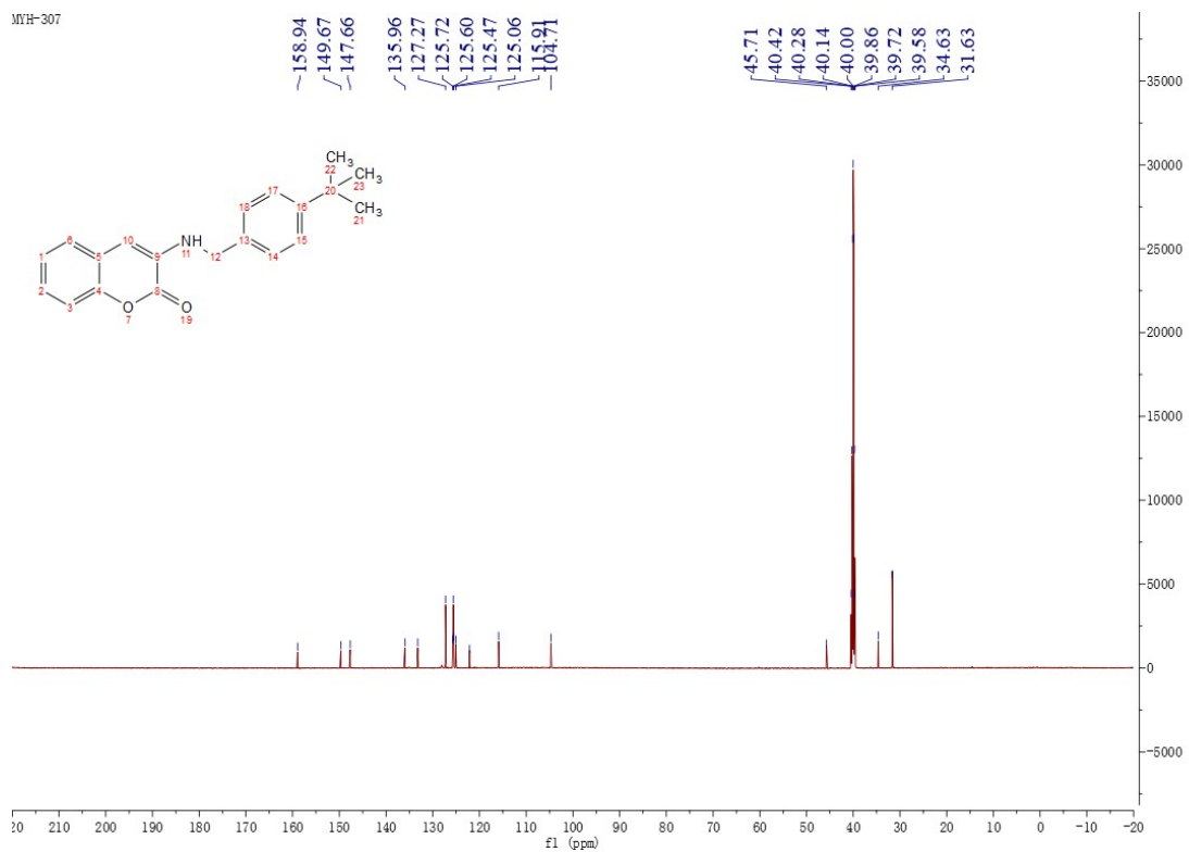
Figure 38 13 C NMR Spectrum of Compound M13
