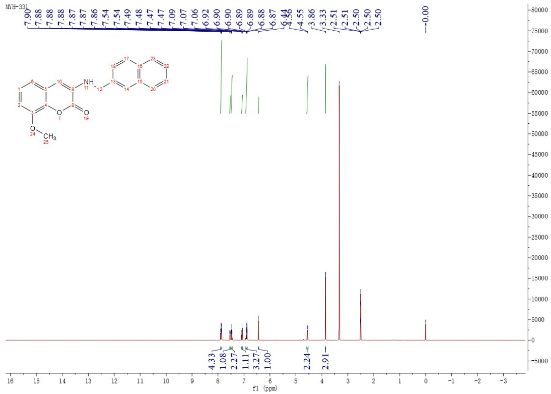
Figure 46 1 H NMR Spectrum of Compound M16
