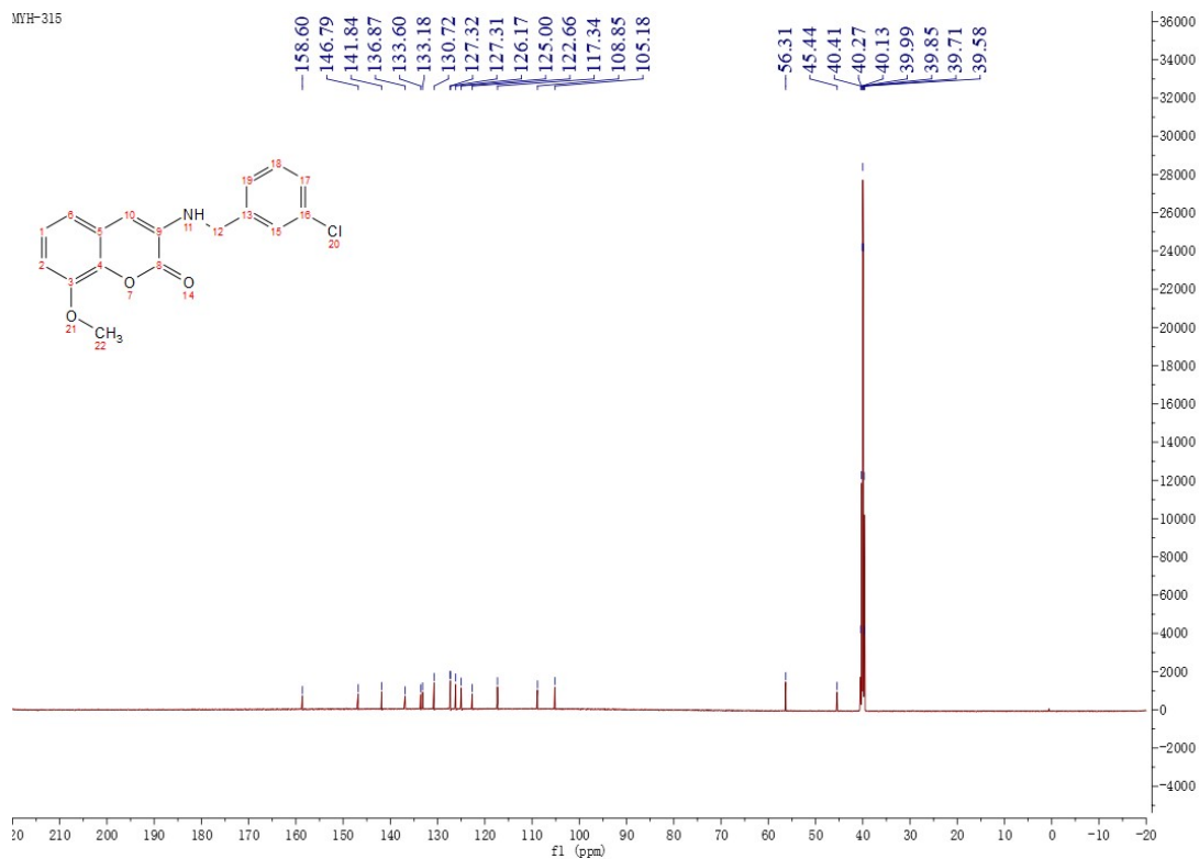
Figure 53 ^{13}\text{C} NMR Spectrum of Compound M18
