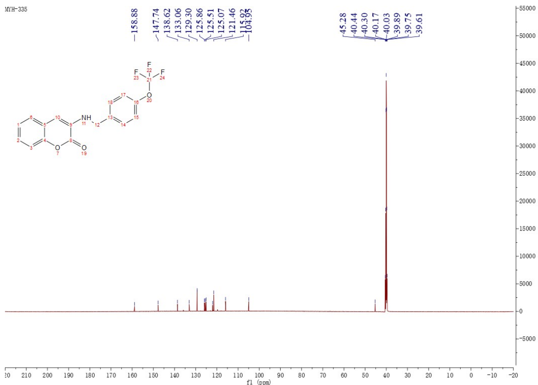
Figure 8 13 C NMR Spectrum of Compound M3
