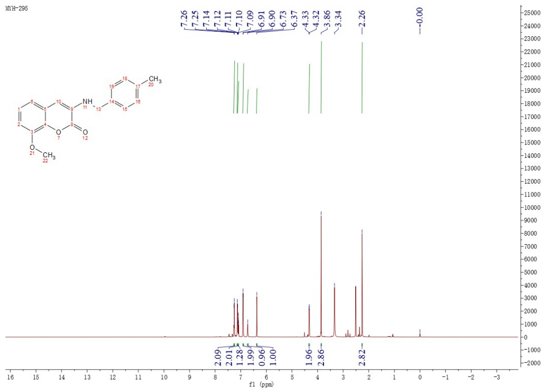
Figure 61 1 H NMR Spectrum of Compound M21
