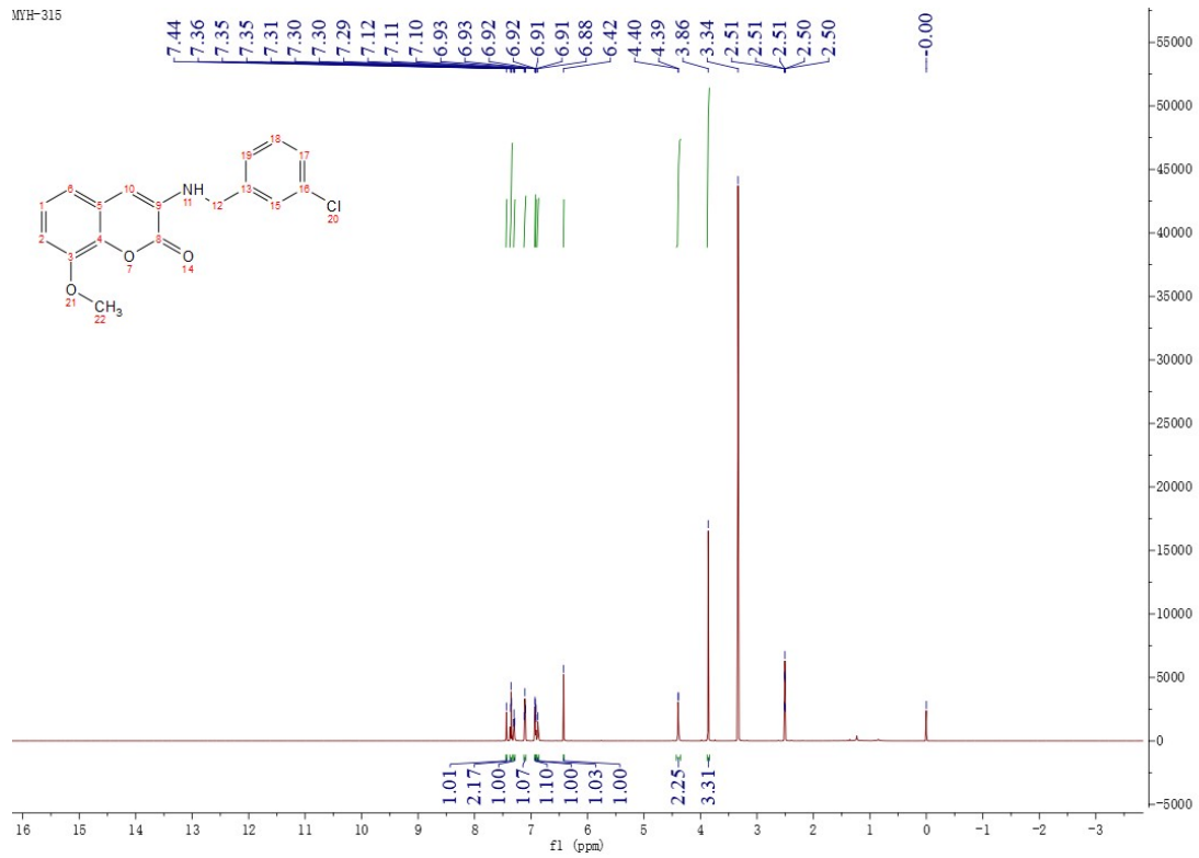
Figure 52 1 H NMR Spectrum of Compound M18
