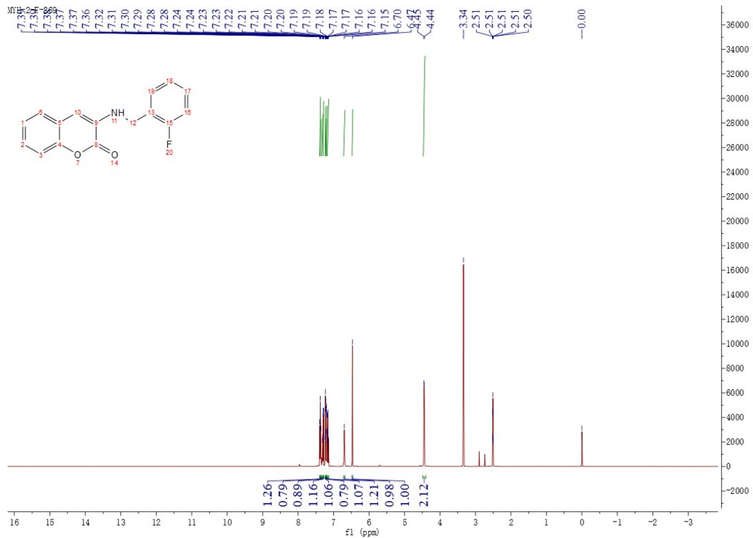
Figure 10 1 H NMR Spectrum of Compound M4
