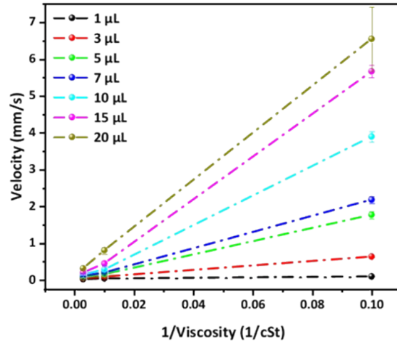
Figure S1. The relationship between the sliding speed of the droplet and the viscosity of the lubricant.
